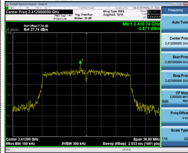
Reference CH01
