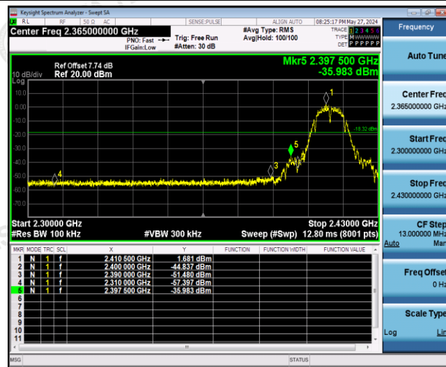
Left bandedge
