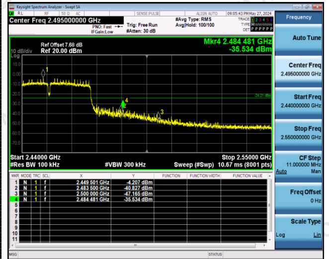
Right bandedge
