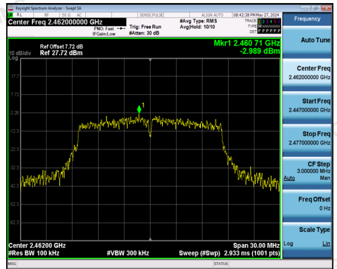
Reference CH11
