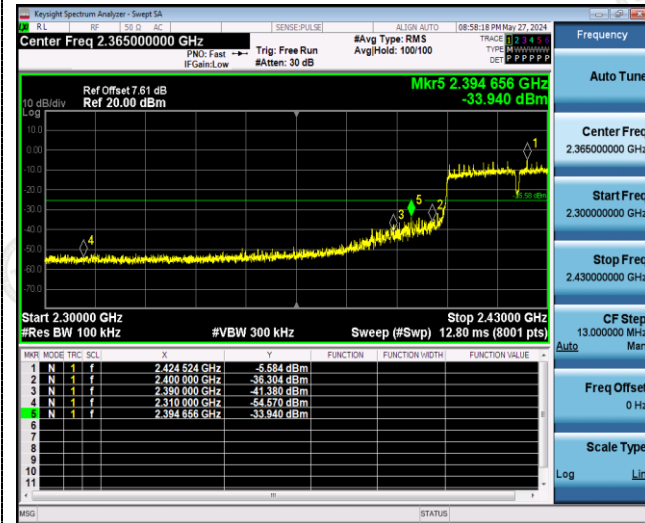
Left bandedge
