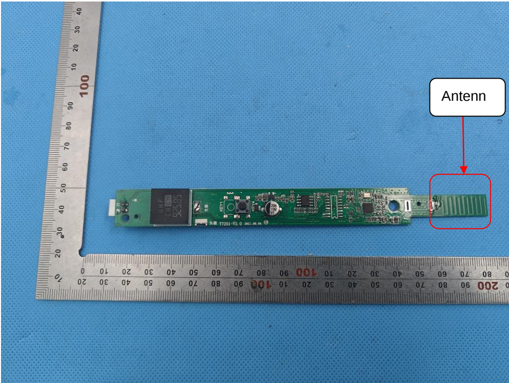
Antenna Diagram 2
