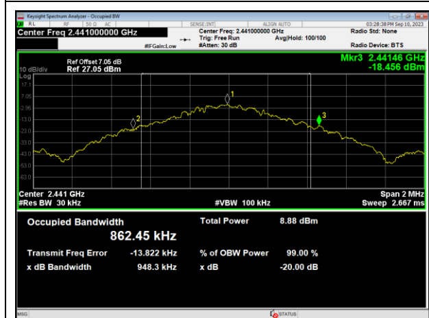
2441MHz
