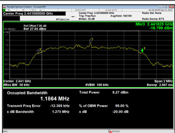
2441MHz
