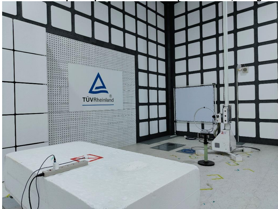
Photograph 14: Test Setup for Spurious Emissions (Back View 1, Charge Mode)
