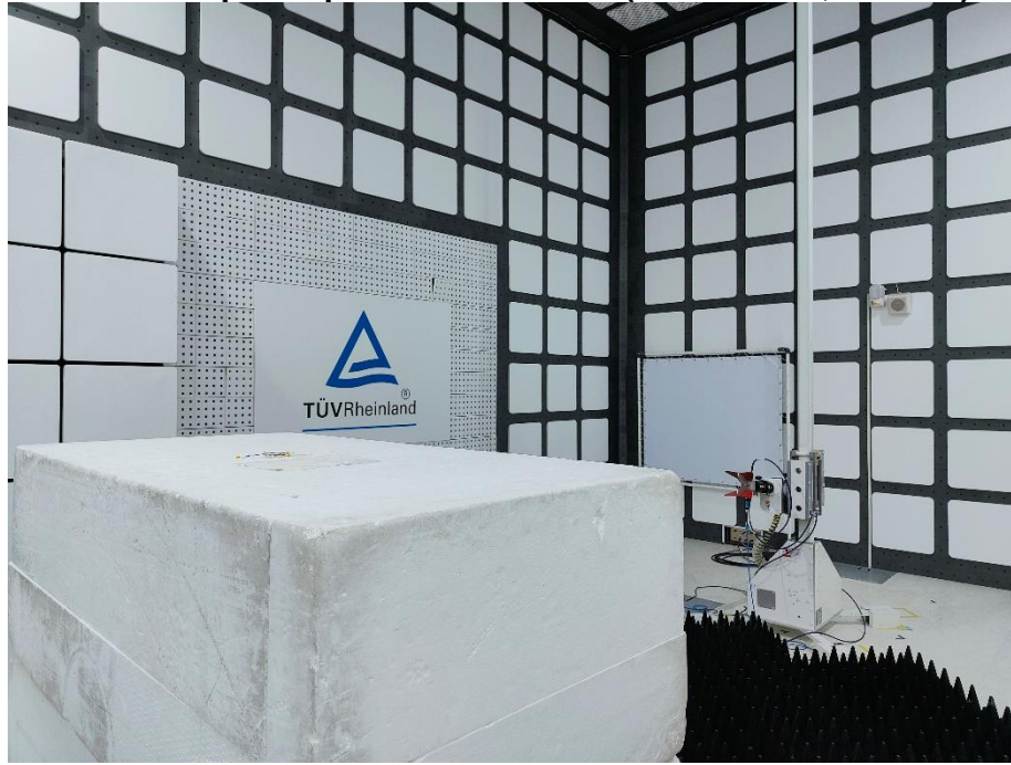
Photograph 6: Test Setup for Spurious Emissions (Back View 4, Left Ear)
