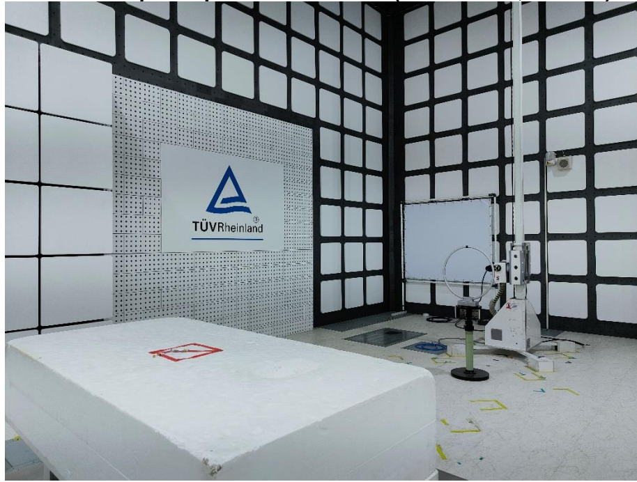
Photograph 4: Test Setup for Spurious Emissions (Back View 2, Left Ear)
