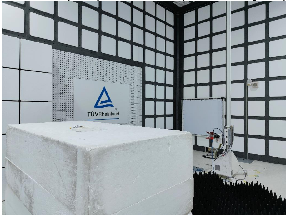
Photograph 12: Test Setup for Spurious Emissions (Back View 4, Right Ear)
