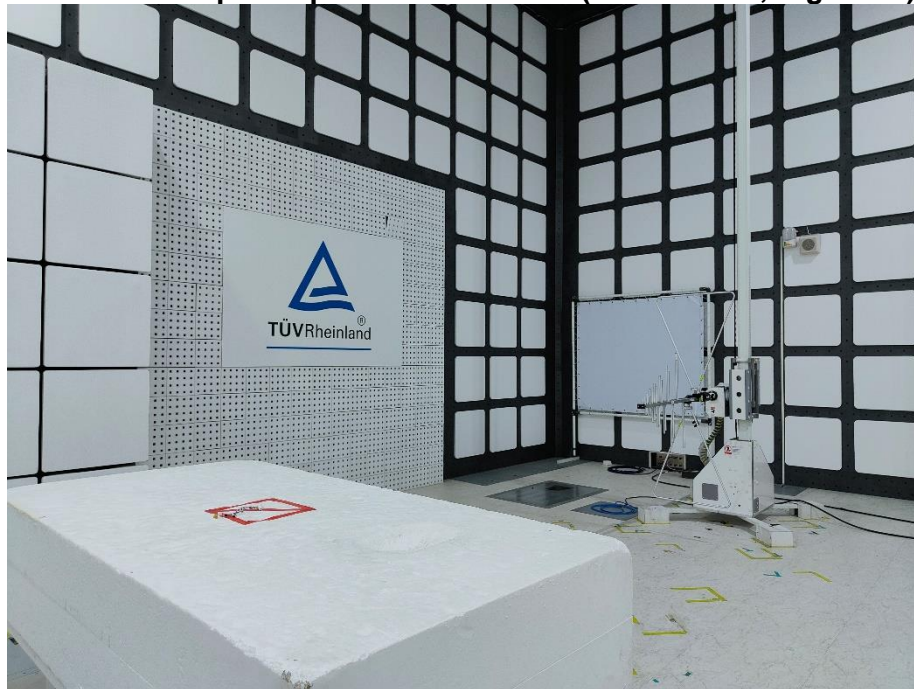
Photograph 10: Test Setup for Spurious Emissions (Back View 2, Right Ear)
