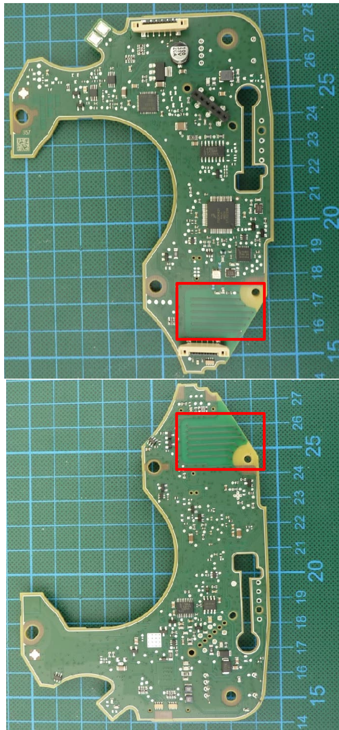
COM 2020, 433 MHz RX antenna position
