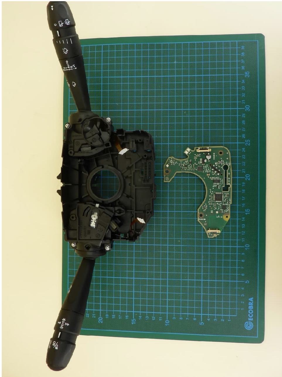
COM 2020, internal view 2, PCB removed
