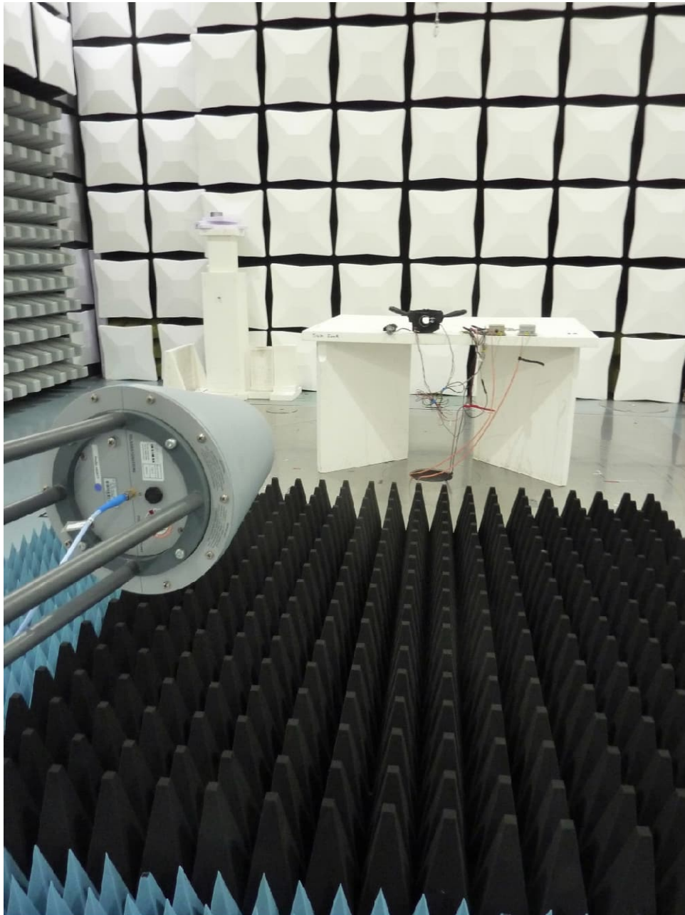
Test setup semi-anechoic chamber M276, 1 – 2 GHz
