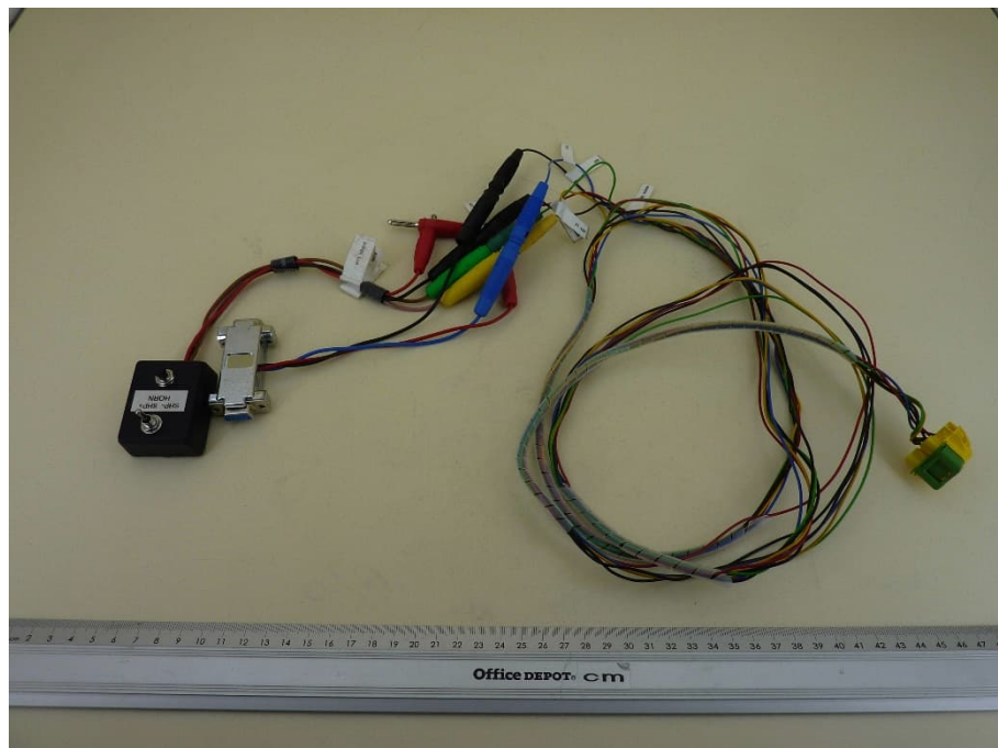
Secondary cable harness (LIN, SHP)
