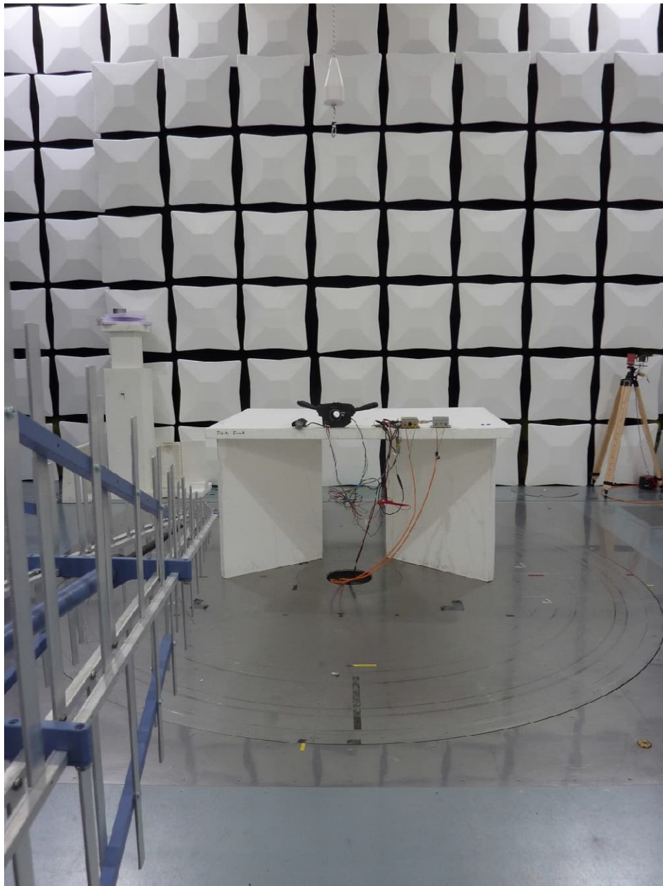
Test setup semi-anechoic chamber M276, 30 MHz – 1 GHz
