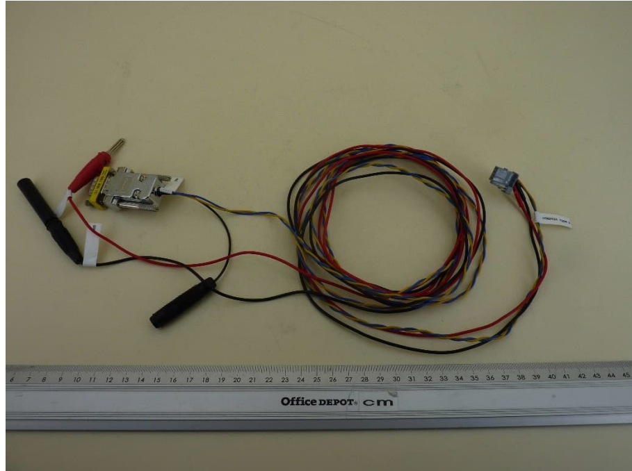
Main cable harness (PWR, CAN)
