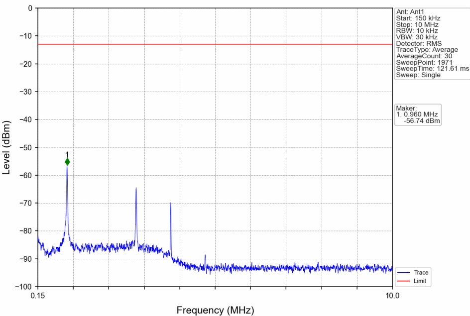
Band5_HSDPA_MCH_836.6MHz_Subtest 1_NTNV
