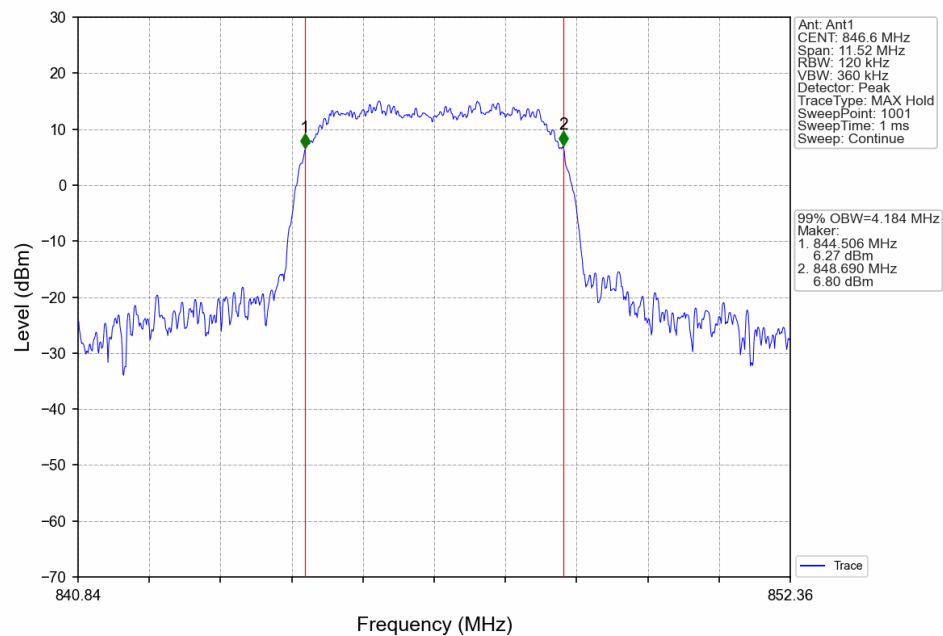
Band5_HSDPA_HCH_846.6MHz_Subtest 1_NTNV
