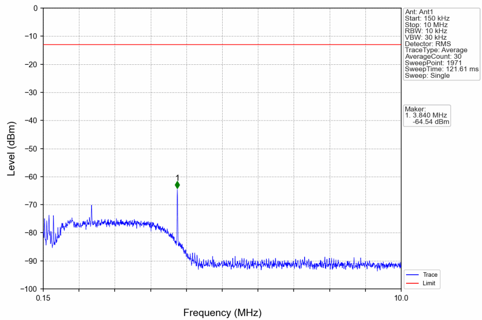
Band4_HSDPA_LCH_1712.4MHz_Subtest 1_NTNV
