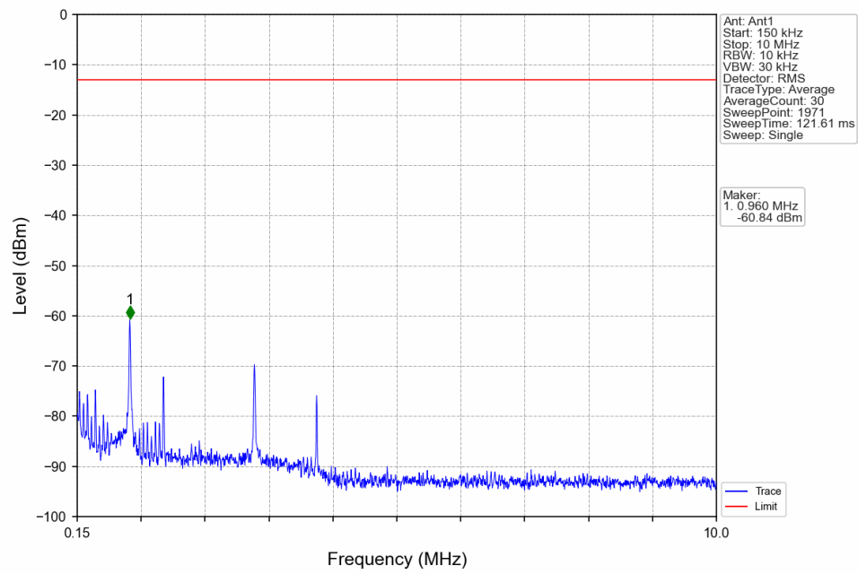
Band2_HSUPA_LCH_1852.4MHz_Subtest 1_NTNV
