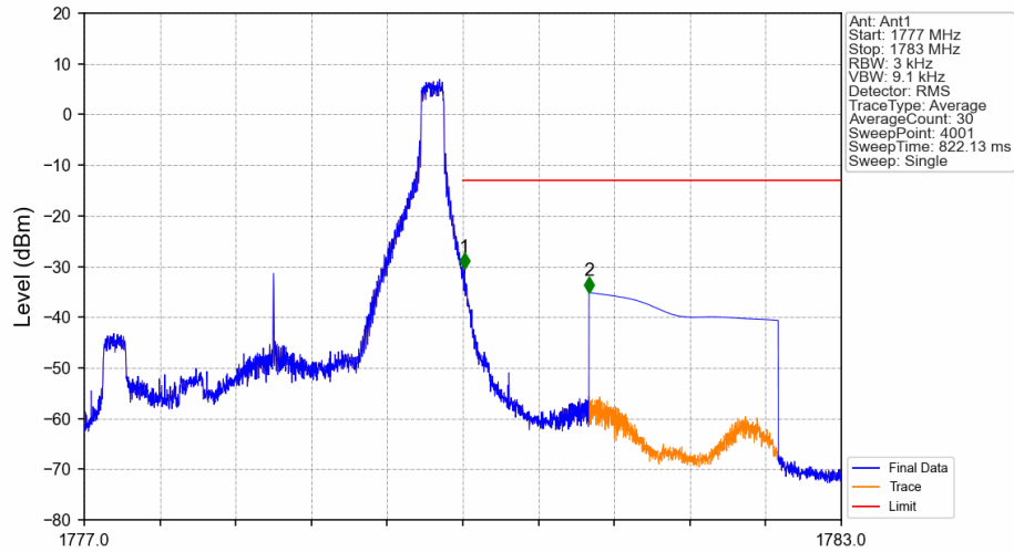
Band66_3MHz_QPSK_HCH_1778.5MHz_RB_1_14_NTNV
