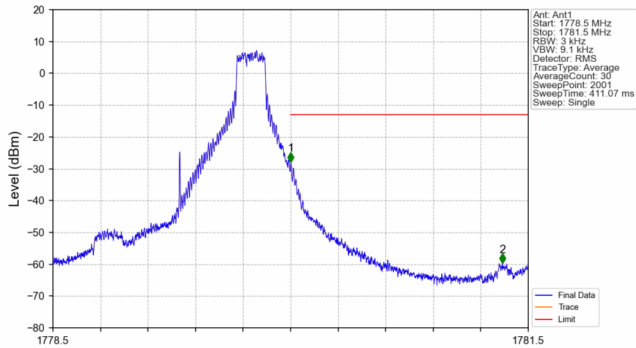
Band66_1.4MHz_QPSK_HCH_1779.3MHz_RB_1_5_NTNV
