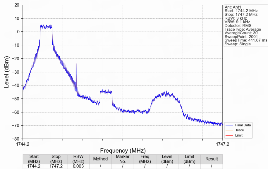
Band66 1.4MHz 16QAM MCH 1745MHz RB 1 0 NTVN
