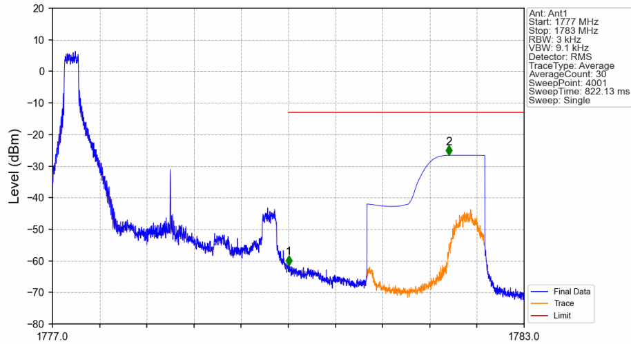
Band66_3MHz_16QAM_HCH_1778.5MHz_RB_1_0_NTNV
