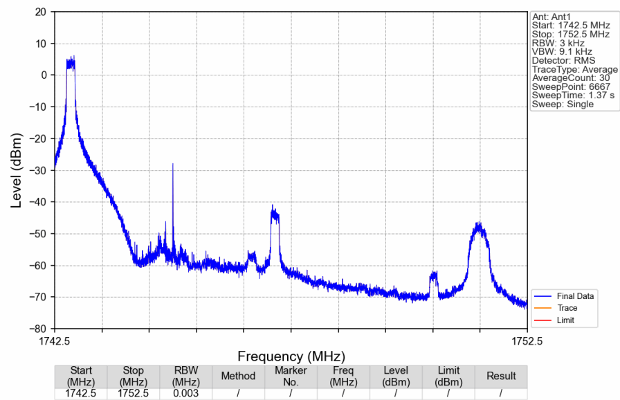
Band66_5MHz_16QAM_MCH_1745MHz_RB_1_0_NTNV
