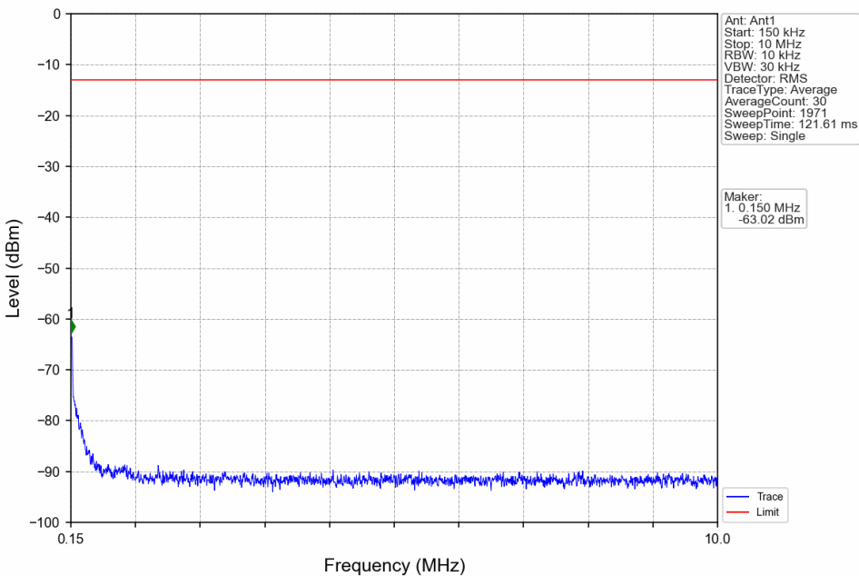
Band66_3MHz_16QAM_MCH_1745MHz_RB_1_0_NTNV
