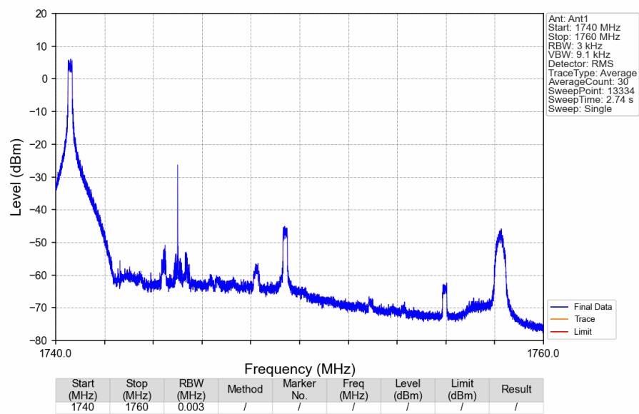
Band66_10MHz_16QAM_MCH_1745MHz_RB_1_0_NTNV
