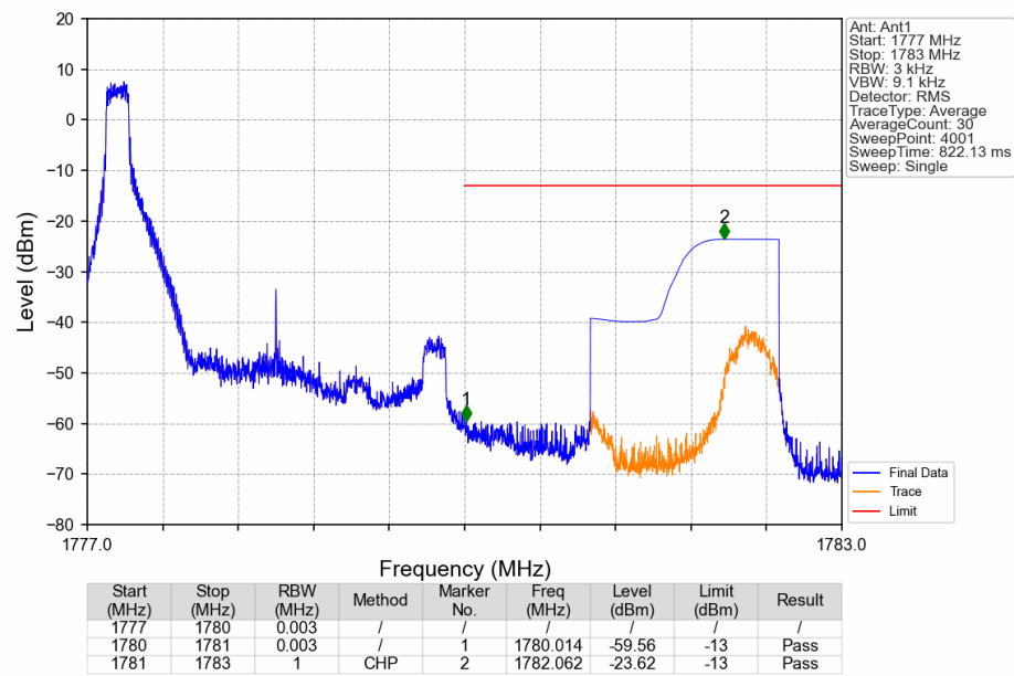
Band66_3MHz_QPSK_HCH_1778.5MHz_RB_1_0_NTNV
