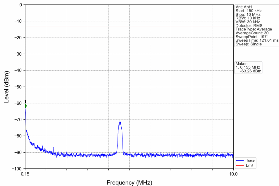
Band66_10MHz_16QAM_LCH_1715MHz_RB_50_0_NTNV
