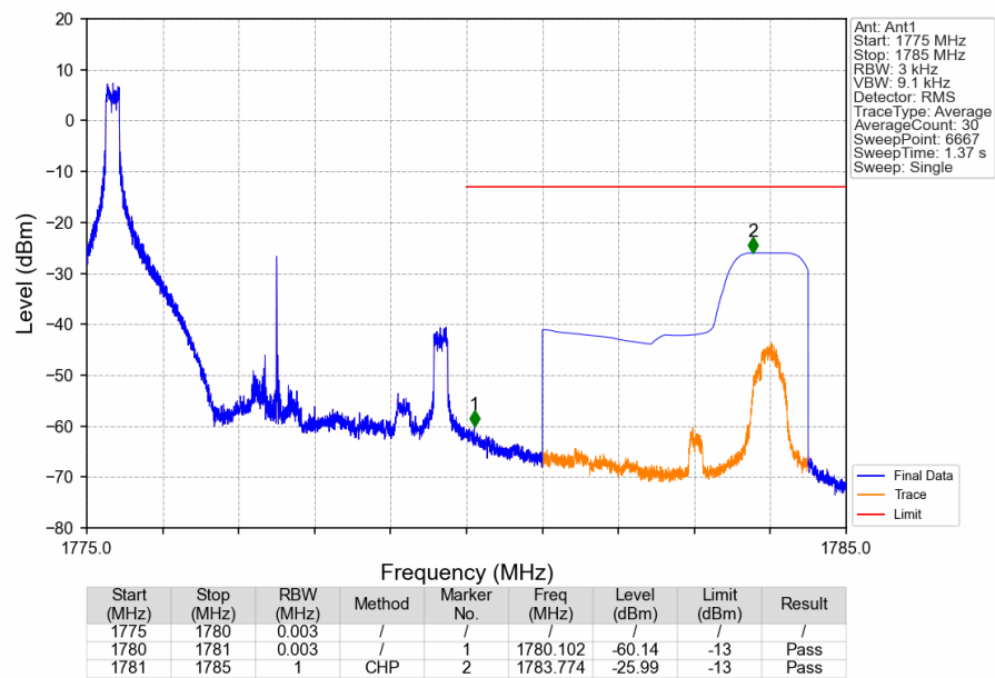
Band66_5MHz_QPSK_HCH_1777.5MHz_RB_1_0_NTNV
