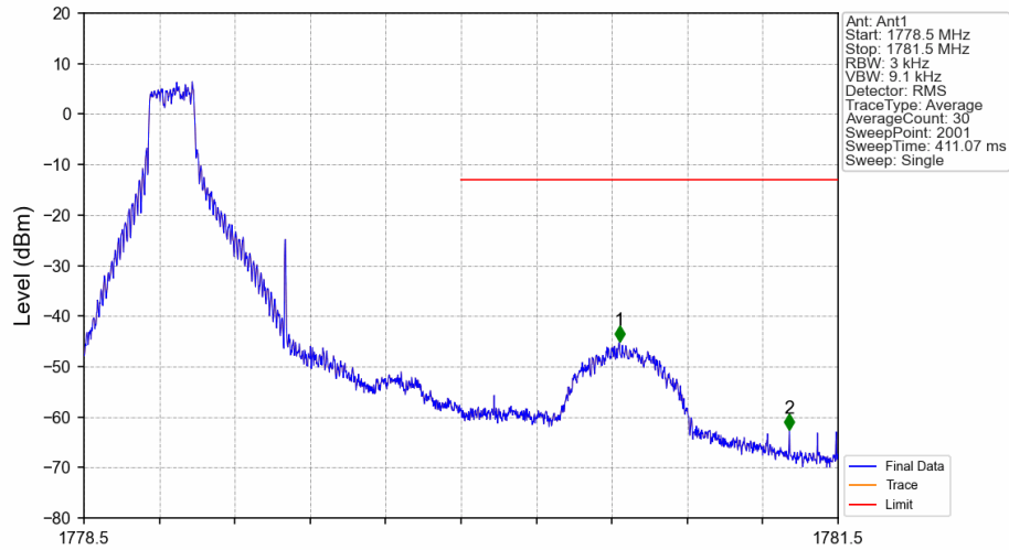
Band66_1.4MHz_16QAM_HCH_1779.3MHz_RB_1_0_NTNV
