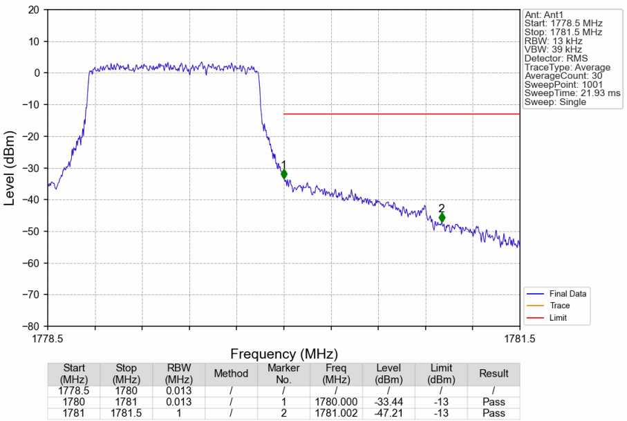
Band66_1.4MHz_16QAM_HCH_1779.3MHz_RB_6_0_NTNV
