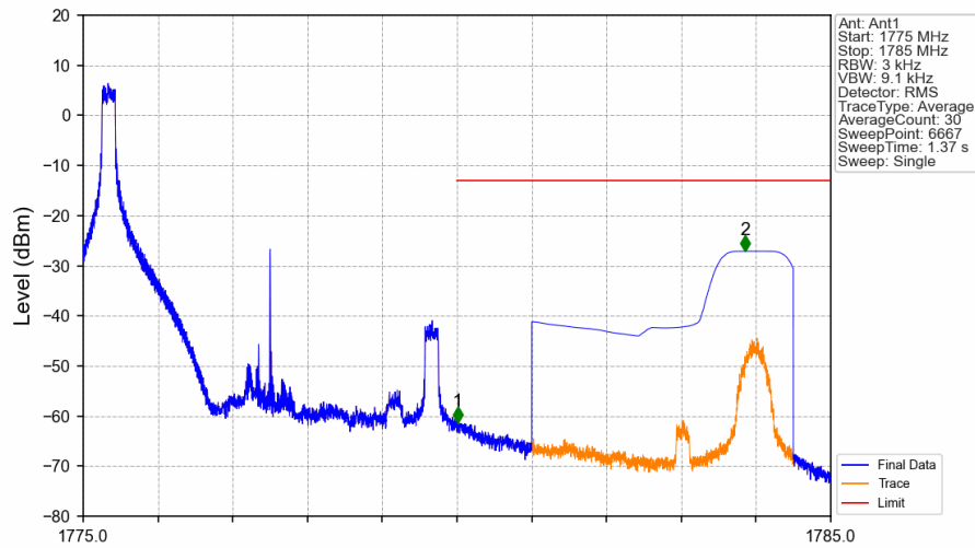
Band66_5MHz_16QAM_HCH_1777.5MHz_RB_1_0_NTNV
