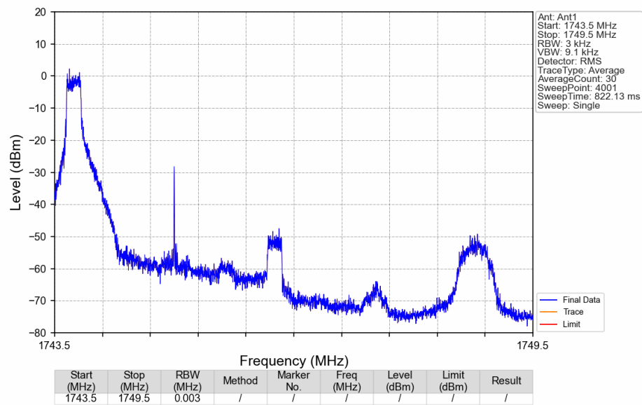
Band66_3MHz_16QAM_MCH_1745MHz_RB_1_0_NTNV
