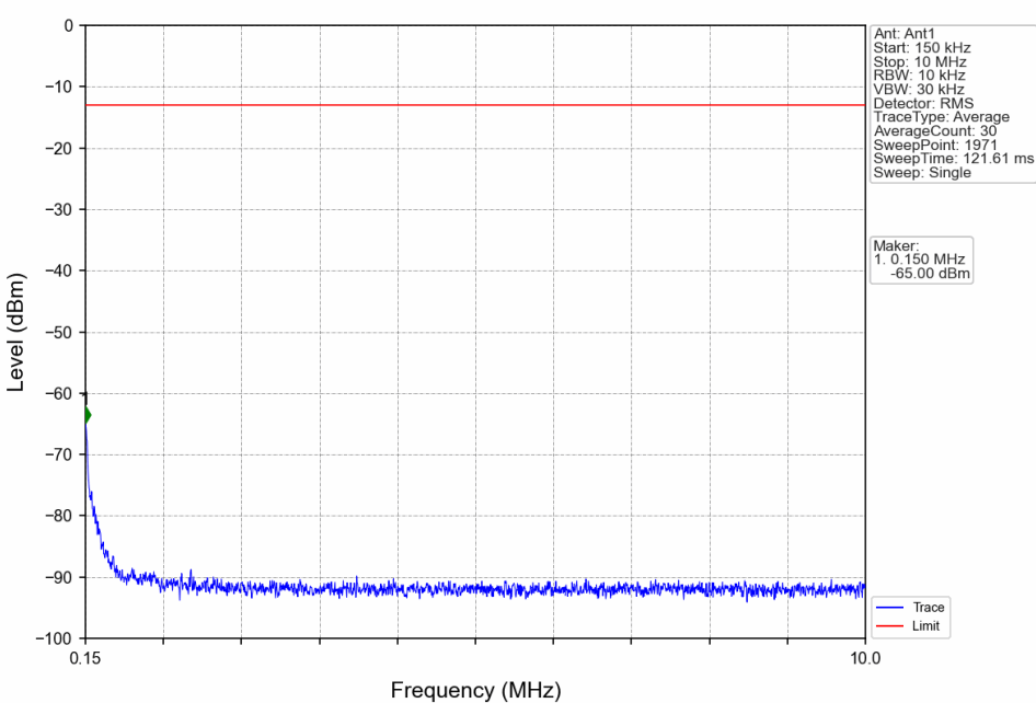
Band66 1.4MHz 16QAM MCH 1745MHz RB 1 0 NTVN
