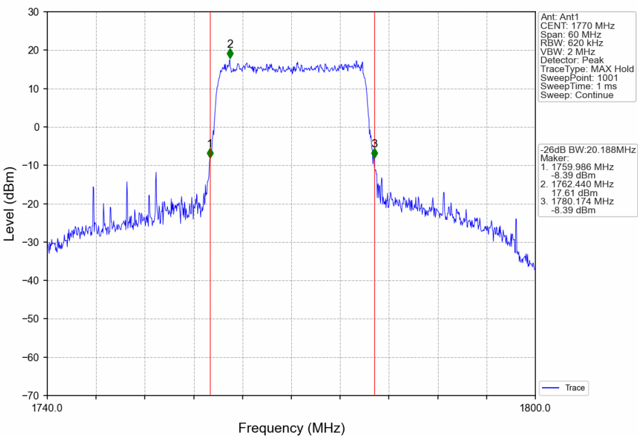
Band66_20MHz_16QAM_HCH_1770MHz_RB_100_0_NTNV
