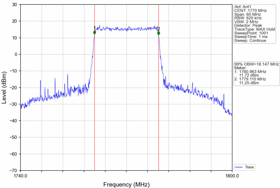
Band66_20MHz_16QAM_HCH_1770MHz_RB_100_0_NTNV
