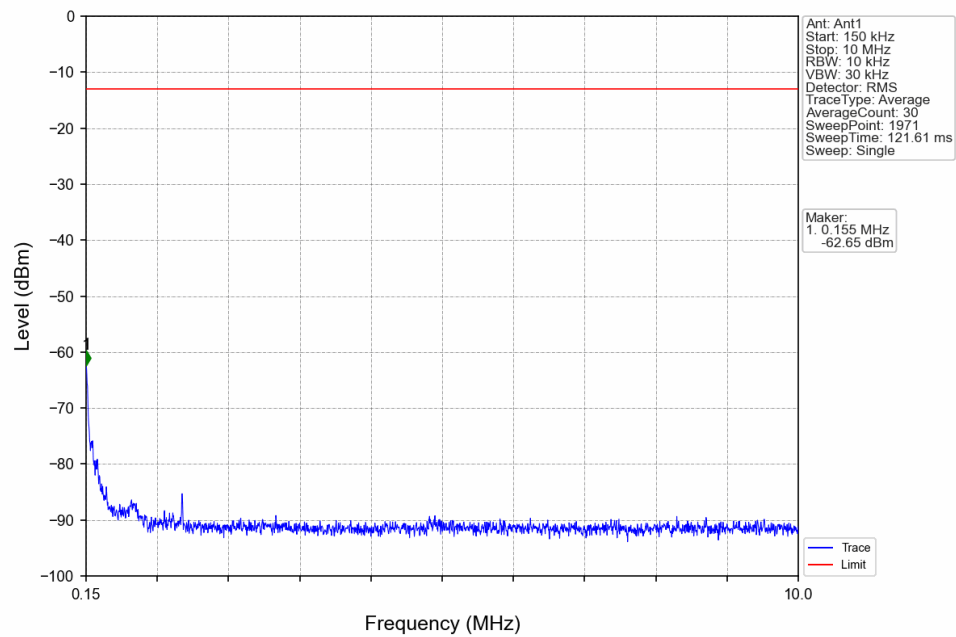
Band5_3MHz_16QAM_LCH_825.5MHz_RB_15_0_NTNV
