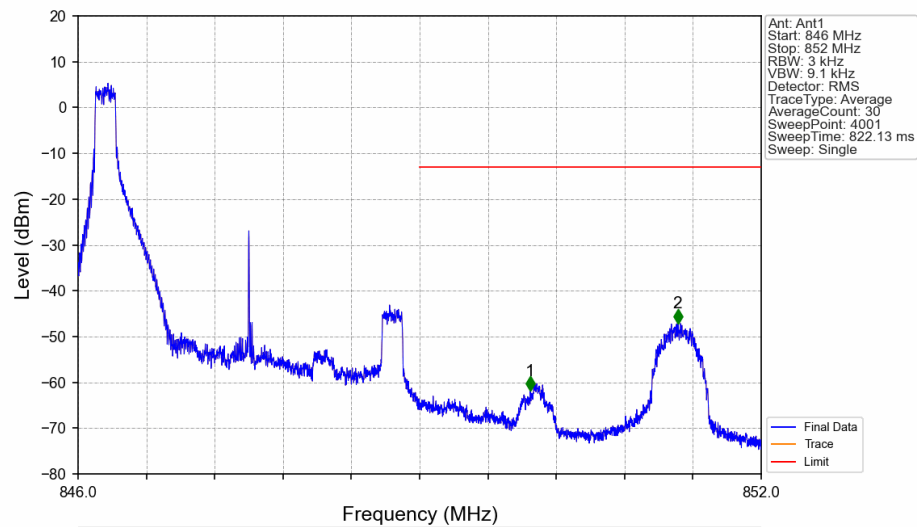
Band5_3MHz_16QAM_HCH_847.5MHz_RB_1_0_NTNV
