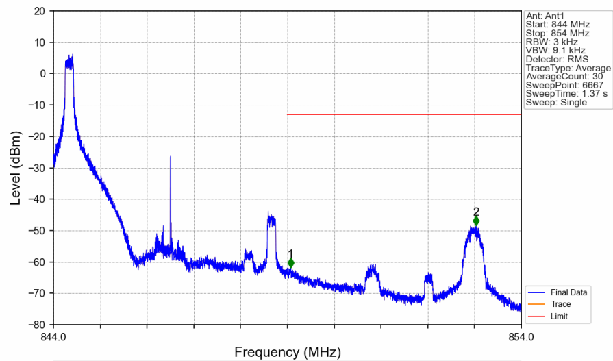
Band5_5MHz_16QAM_HCH_846.5MHz_RB_1_0_NTNV
