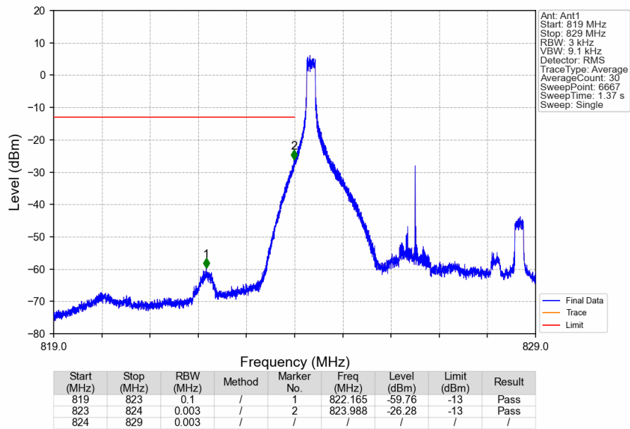
Band5_5MHz_16QAM_LCH_826.5MHz_RB_1_0_NTNV
