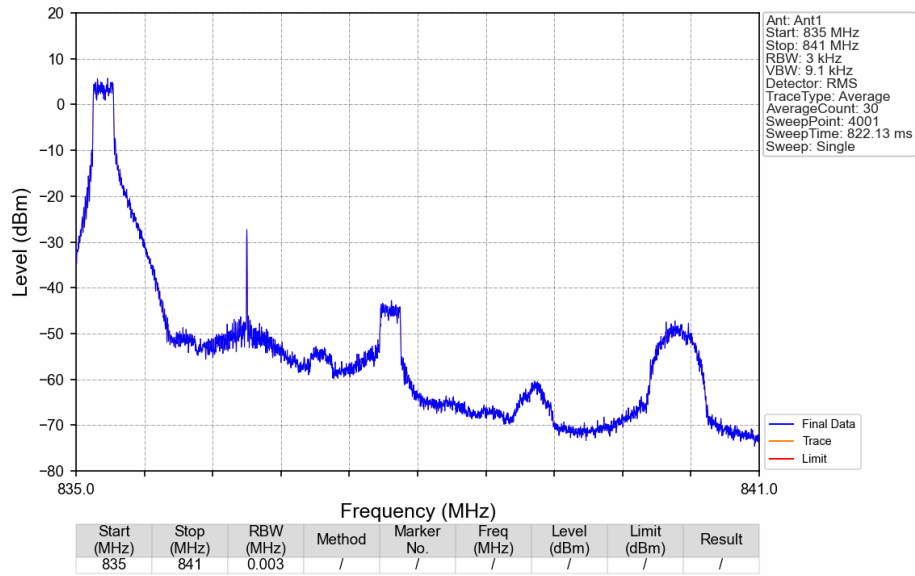
Band5_3MHz_16QAM_MCH_836.5MHz_RB_1_0_NTNV
