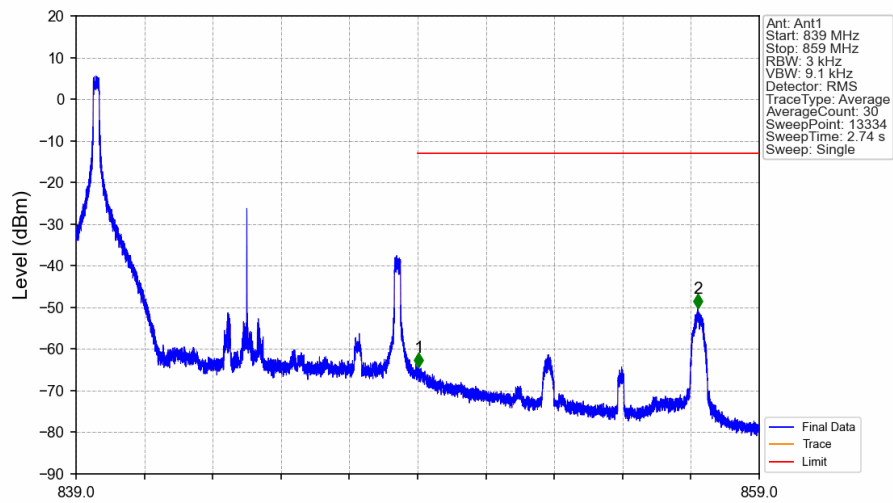
Band5_10MHz_16QAM_HCH_844MHz_RB_1_0_NTNV
