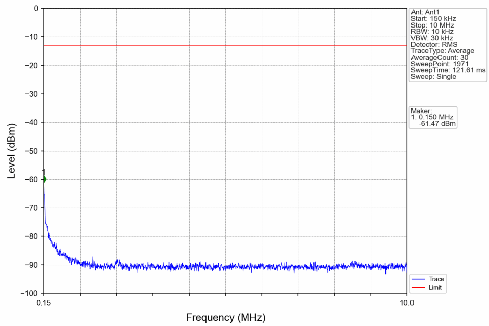
Band5_5MHz_QPSK_MCH_836.5MHz_RB_1_0_NTNV
