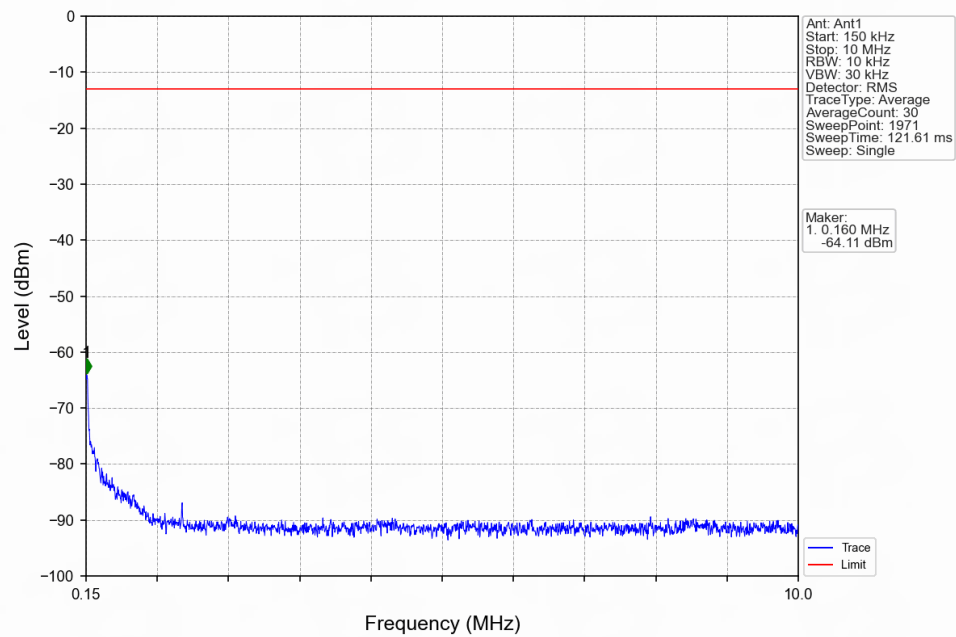
Band5_5MHz_16QAM_LCH_826.5MHz_RB_25_0_NTNV
