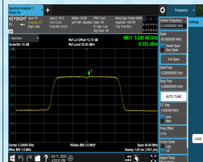
11AC20MIMO-Ant1-5240-PASS
