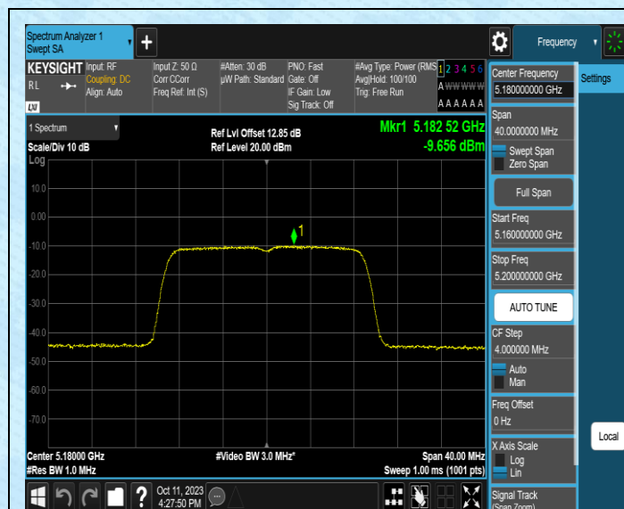
11AC20MIMO-Ant1-5180-PASS
