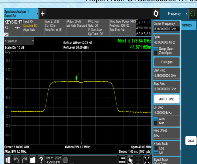
11AC20MIMO-Ant2-5180-PASS
