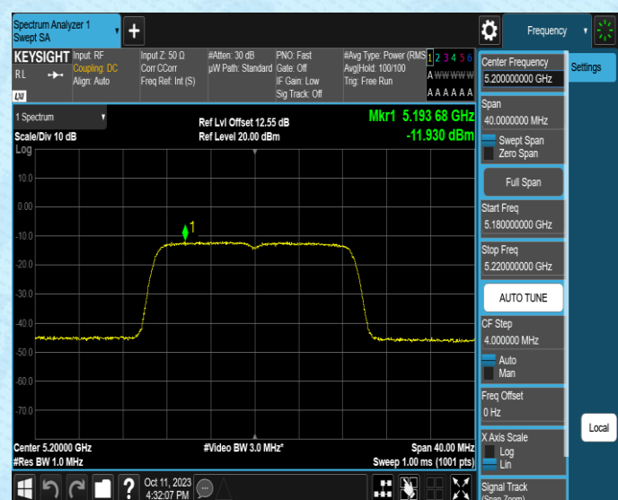
11AC20MIMO-Ant2-5200-PASS
