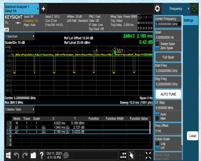
NTNV-11AC20SISO-Ant2-5200
