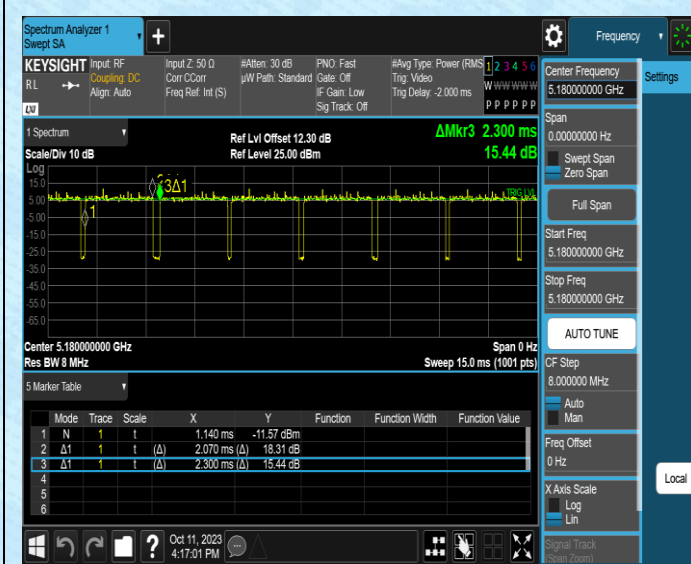
NTNV-11N20MIMO-Ant1-5180
