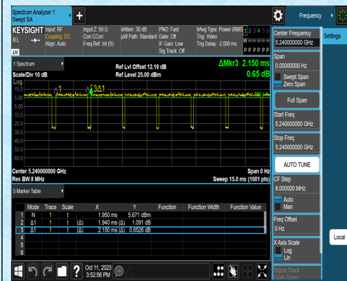
NTNV-11AC20SISO-Ant1-5240
