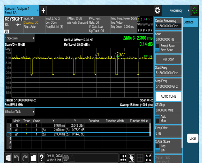
NTNV-11N20MIMO-Ant2-5180
