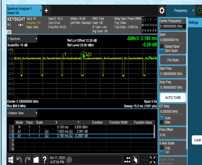
NTNV-11AC20MIMO-Ant1-5180
