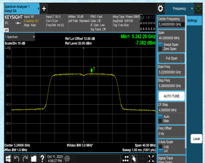
11N20SISO-Ant2-5240-PASS
