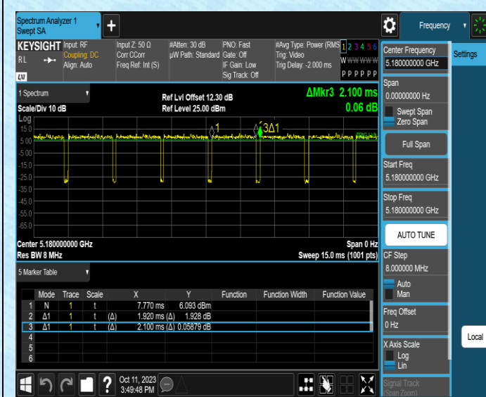
NTNV-11AC20SISO-Ant1-5180
