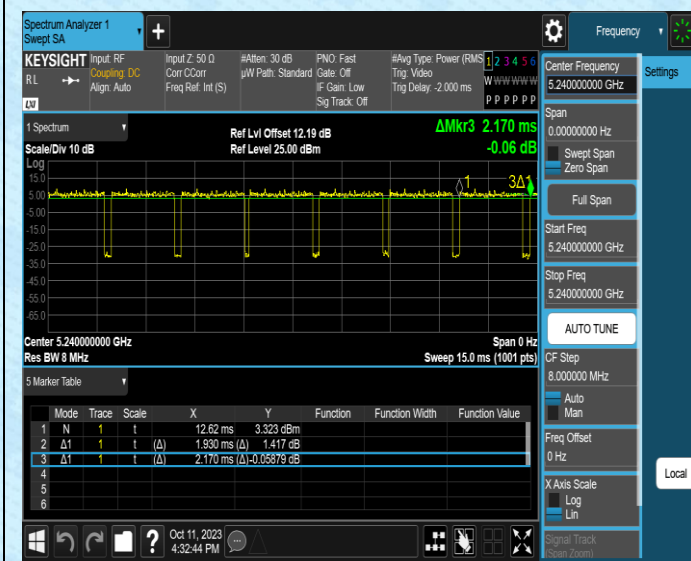
NTNV-11AC20MIMO-Ant1-5240
