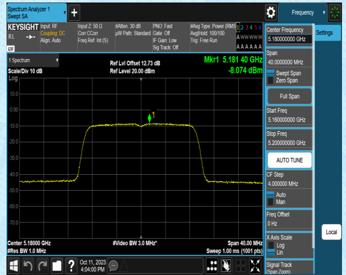
11N20SISO-Ant2-5180-PASS
