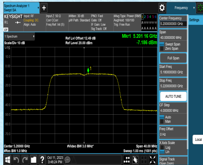
11N20SISO-Ant1-5200-PASS
