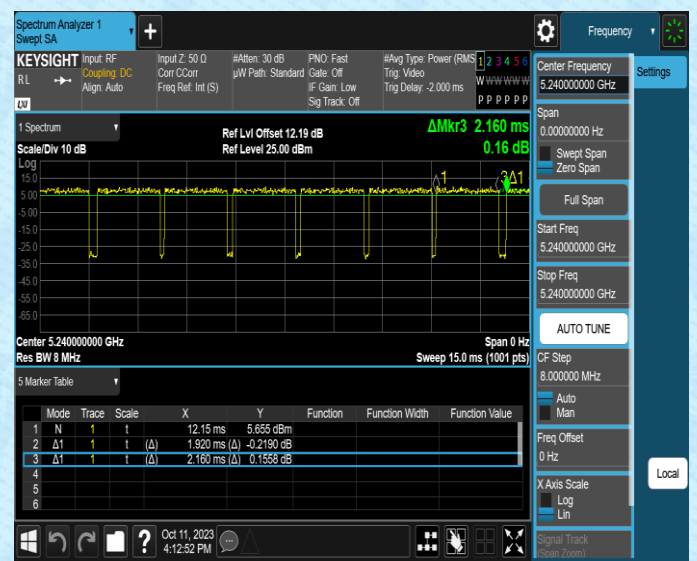
NTNV-11AC20SISO-Ant2-5240
