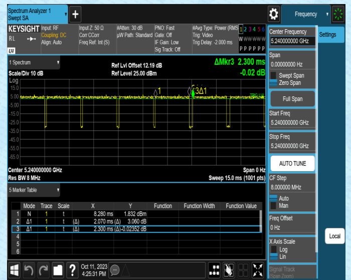
NTNV-11N20MIMO-Ant2-5240
