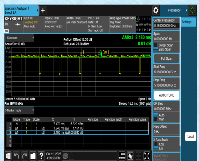
NTNV-11AC20SISO-Ant2-5180
