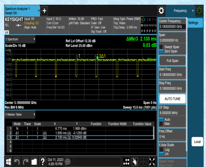
NTNV-11AC20MIMO-Ant2-5180
