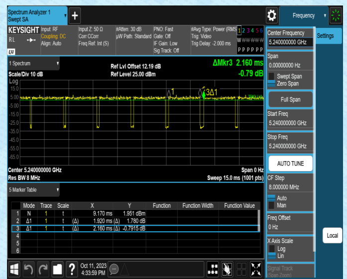
NTNV-11AC20MIMO-Ant2-5240
