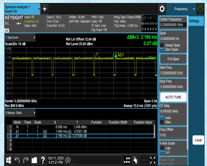
NTNV-11AC20MIMO-Ant2-5200
