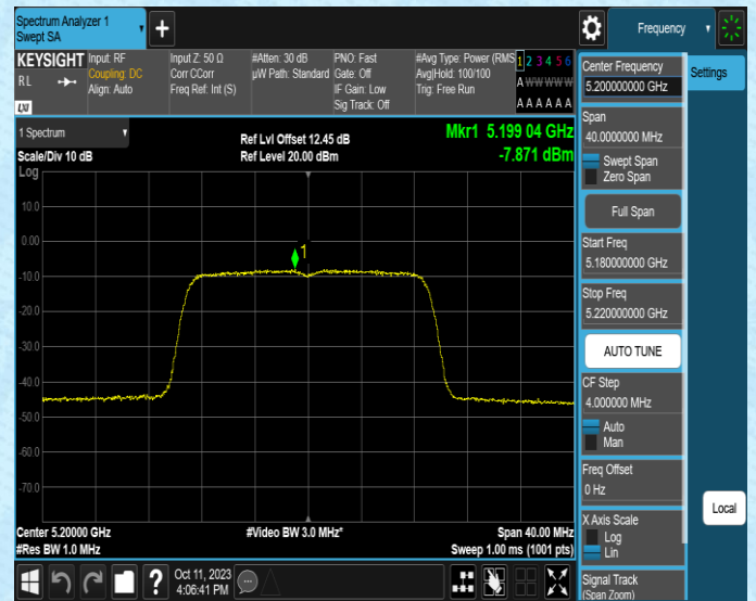
11N20SISO-Ant2-5200-PASS
