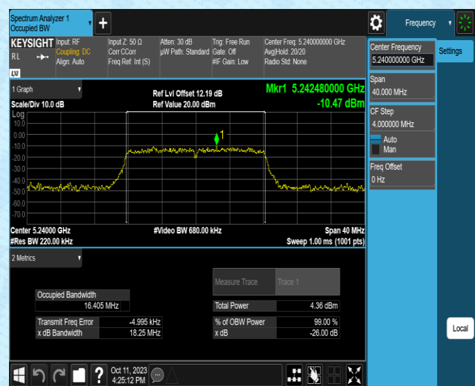
11N20MIMO-Ant2-5240
