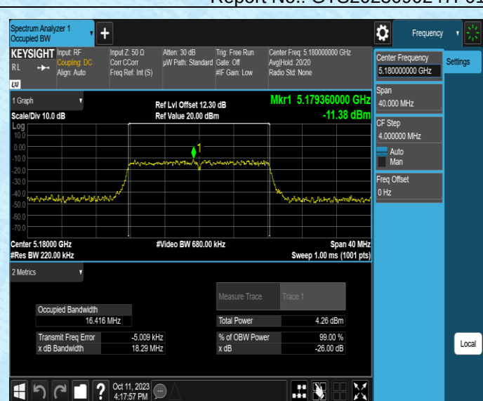
11N20MIMO-Ant2-5180
