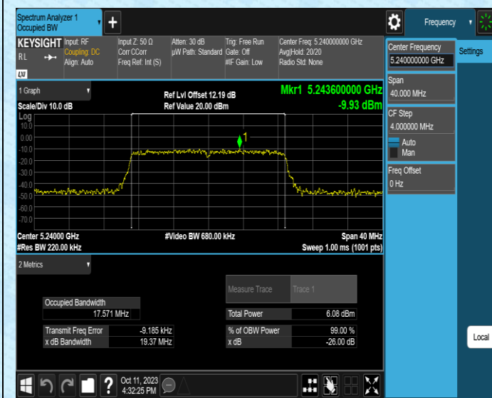
11AC20MIMO-Ant1-5240
