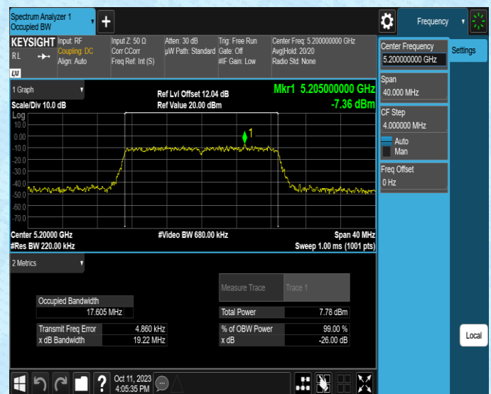
11N20SISO-Ant2-5200
