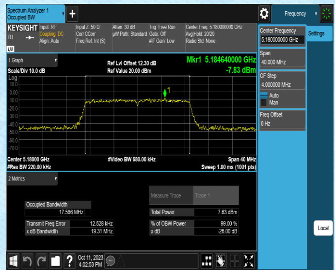
11N20SISO-Ant2-5180
