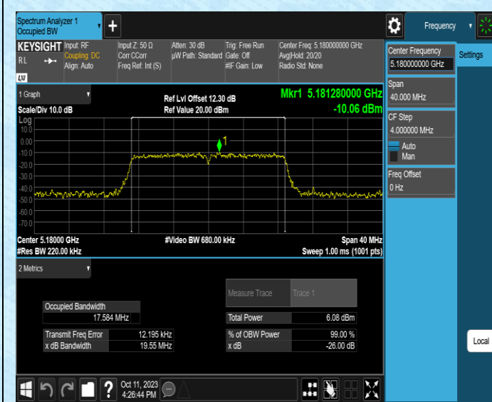
11AC20MIMO-Ant1-5180
