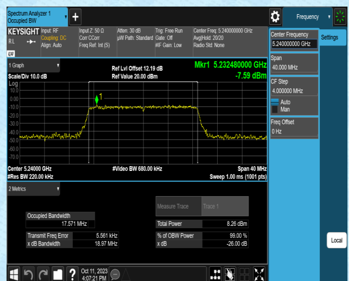
11N20SISO-Ant2-5240
