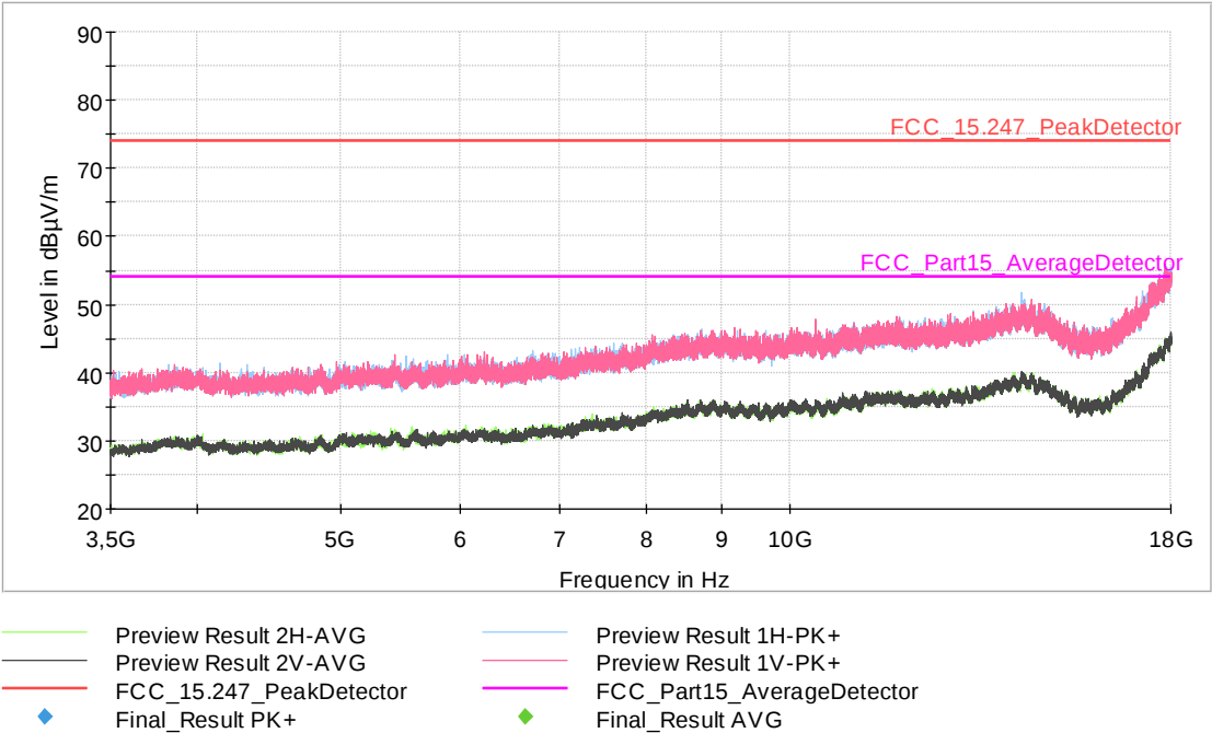
Fig. 30: Ambient level. Frequency range: 3.5 GHz – 18 GHz
