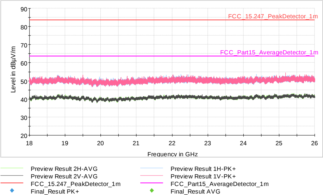
Fig. 31: Ambient level. Frequency range: 18 GHz – 26 GHz
