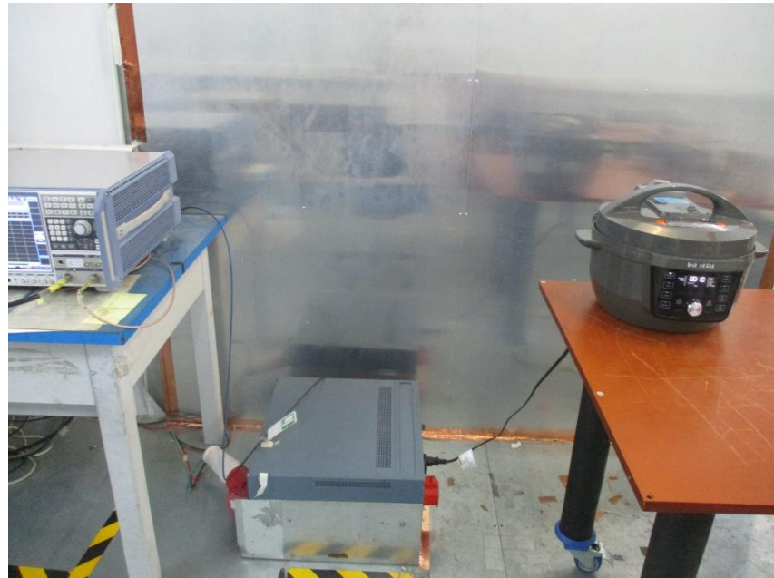
Photograph 3: Set-up for Conducted Emissions
