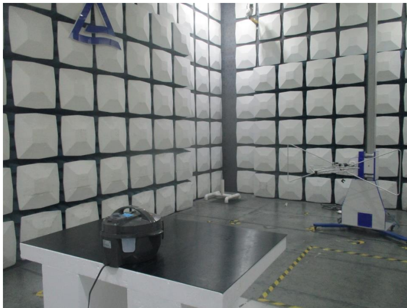
Photograph 2: Set-up for Radiated Spurious Emissions, above 30MHz
