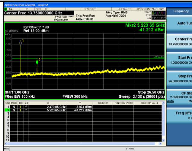
3DH5-Ant1-2480-1000~26500--10.34
