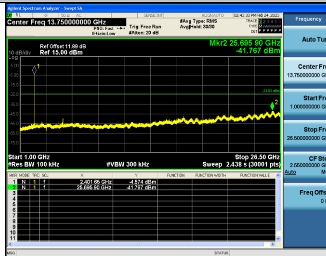
2DH5-Ant1-2441-0~Reference--4.22
