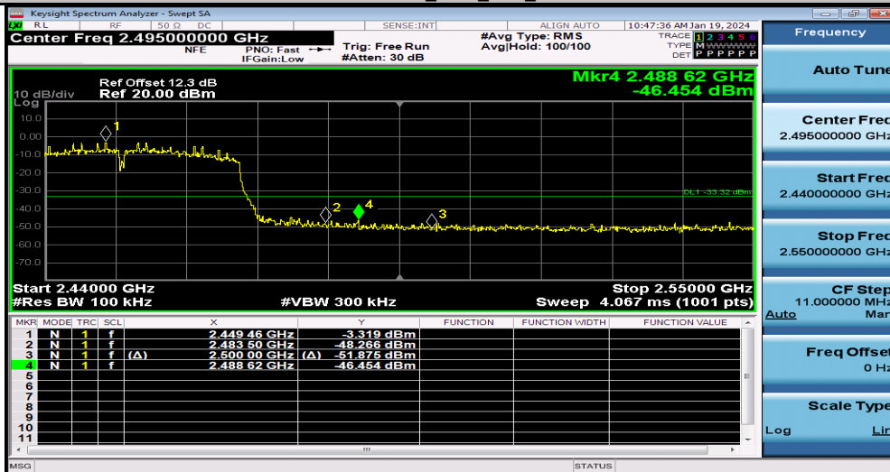
11N40SISO_Ant1_High_2452
