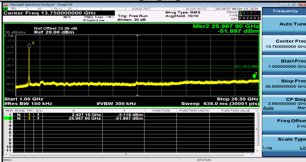
11N40SISO_Ant1_2422_1000~26500
