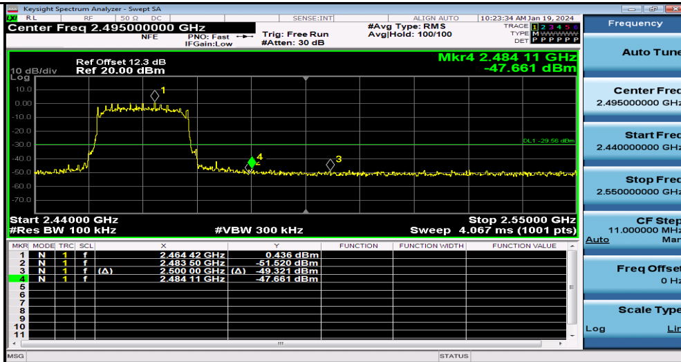
11N20SISO_Ant1_High_2462
