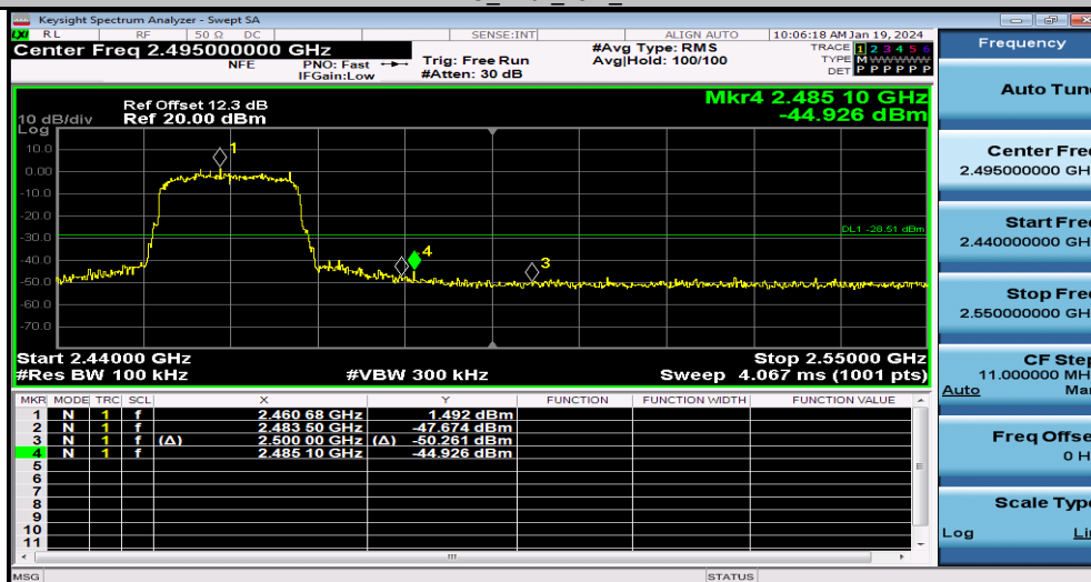
11G_Ant1_High_2462
