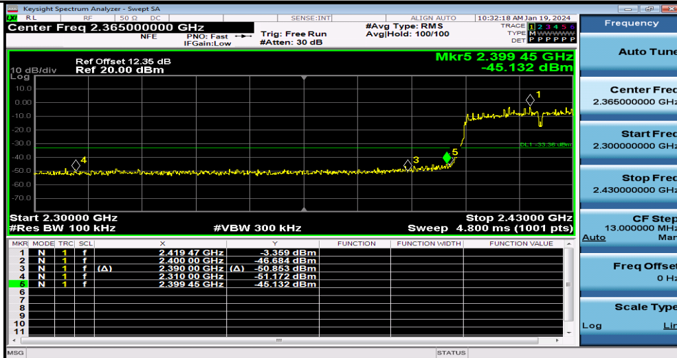
11N40SISO_Ant1_Low_2422
