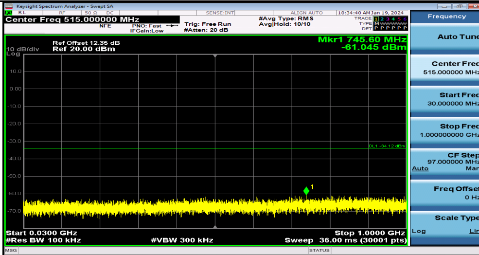
11N40SISO_Ant1_2422_30~1000
