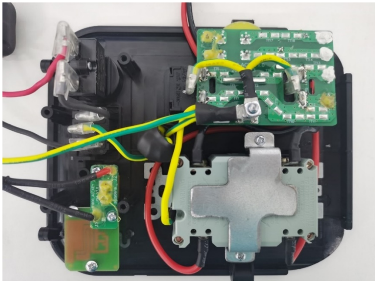
Input/output panel
