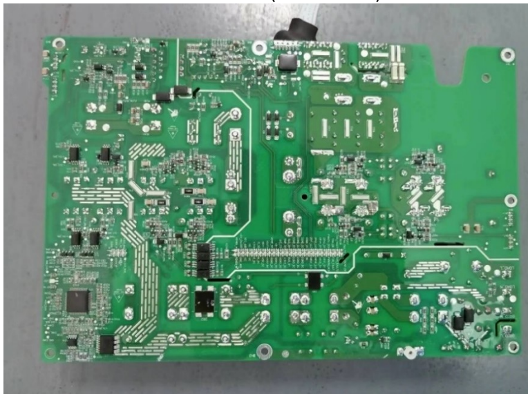
Invertor board(bottom view)
