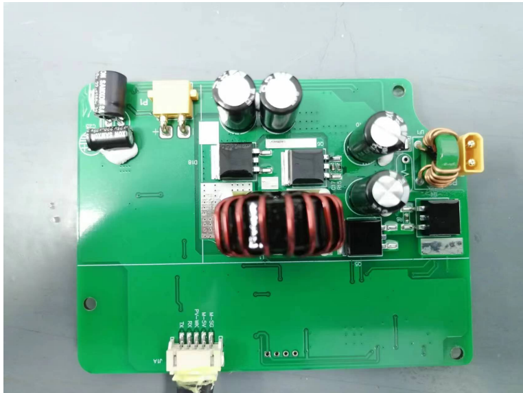
MPPT board
