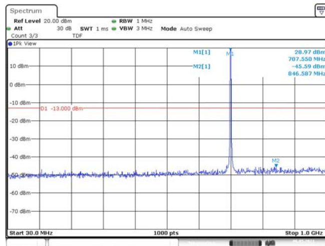
Band12-1.4MHz-QPSK-23095-1RB#0-Range1:30~1000MHz
