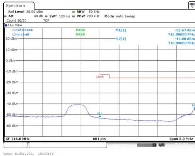
Band12-3MHz-16QAM-23165-1RB#14
