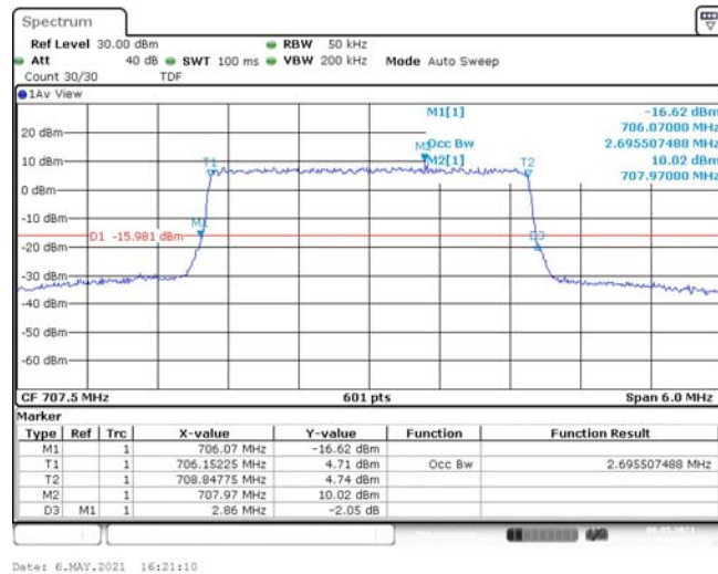
Band12-3MHz-16QAM-23165-15RB#0-2.696
