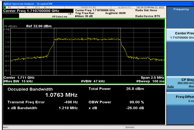
Band4-1.4MHz-16QAM-19957-6RB#0-1.0763
