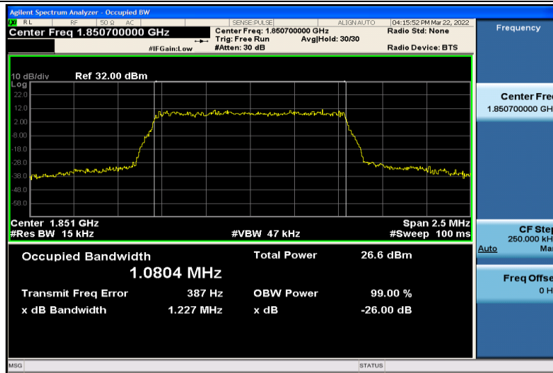
Band2-1.4MHz-16QAM-18607-6RB#0-1.0804
