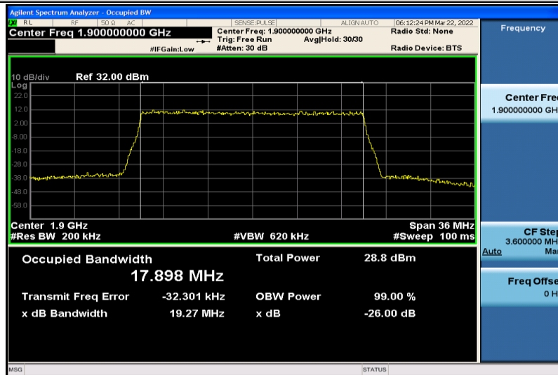
Band2-20MHz-QPSK-19100-100RB#0-17.898
