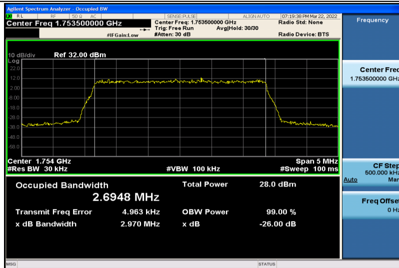
Band4-3MHz-QPSK-20385-15RB#0-2.6948
