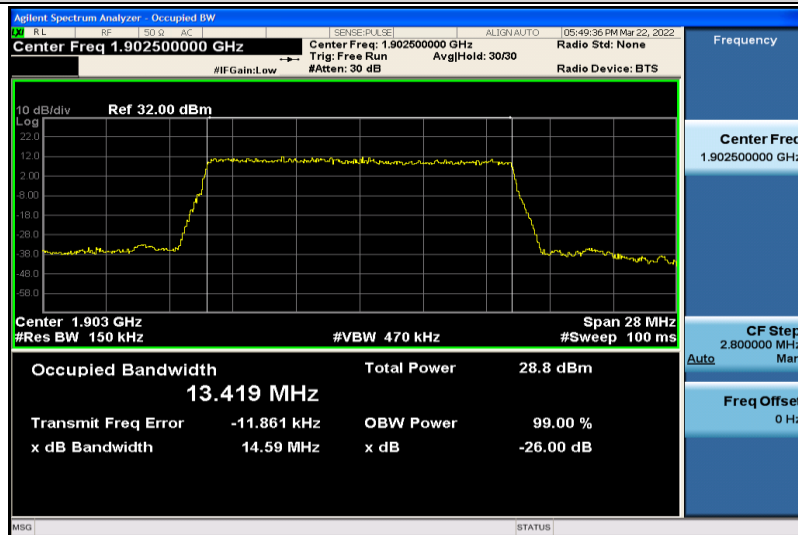
Band2-15MHz-QPSK-19125-75RB#0-13.419
