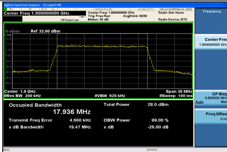
Band2-20MHz-16QAM-19100-100RB#0-17.936
