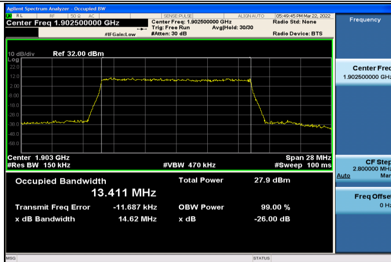
Band2-15MHz-16QAM-19125-75RB#0-13.411
