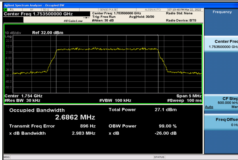
Band4-3MHz-16QAM-20385-15RB#0-2.6862
