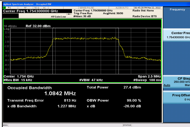
Band4-1.4MHz-QPSK-20393-6RB#0-1.0842
