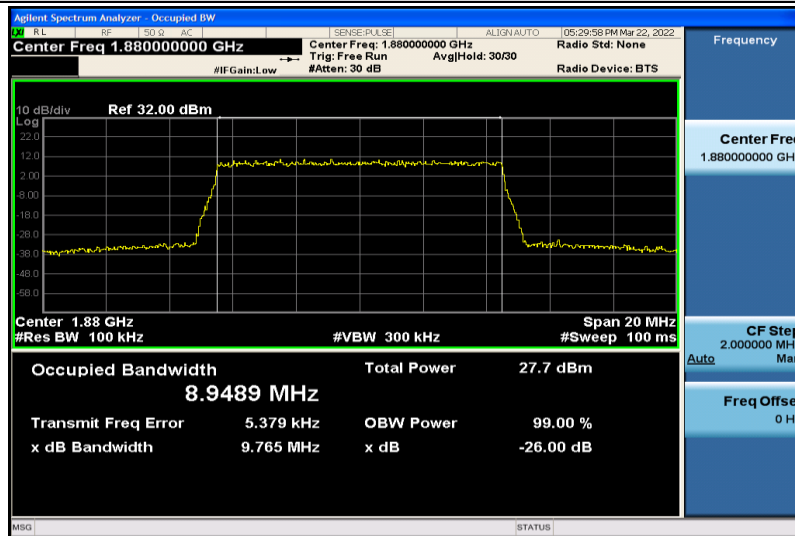
Band2-10MHz-16QAM-18900-50RB#0-8.9489
