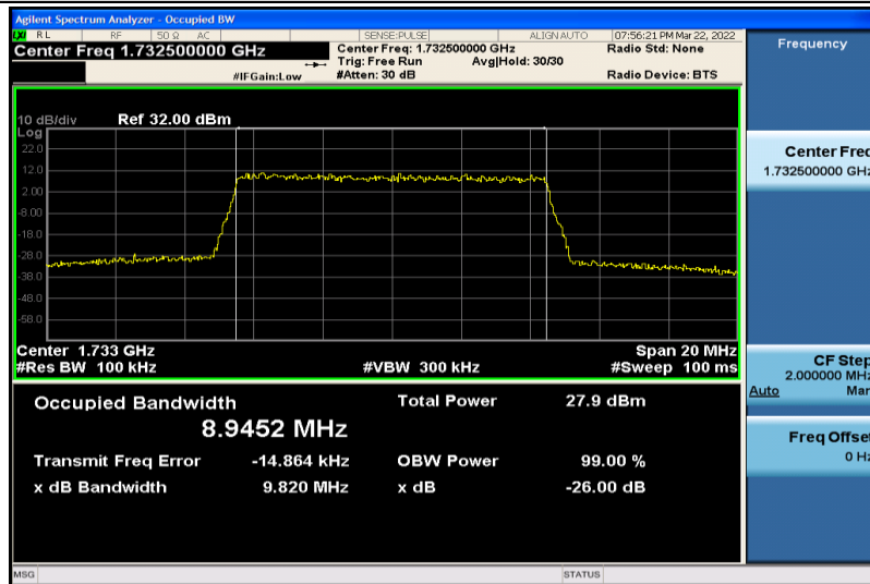
Band4-10MHz-16QAM-20175-50RB#0-8.9452
