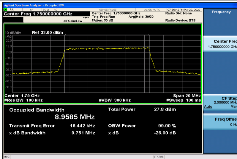
Band4-10MHz-16QAM-20350-50RB#0-8.9585
