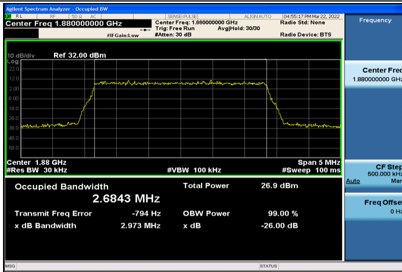
Band2-3MHz-16QAM-18900-15RB#0-2.6843
