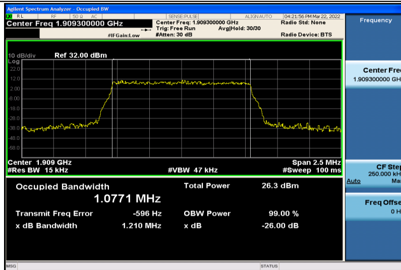
Band2-1.4MHz-16QAM-19193-6RB#0-1.0771
