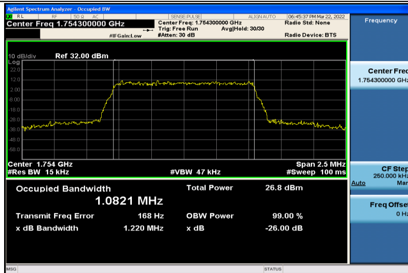
Band4-1.4MHz-16QAM-20393-6RB#0-1.0821
