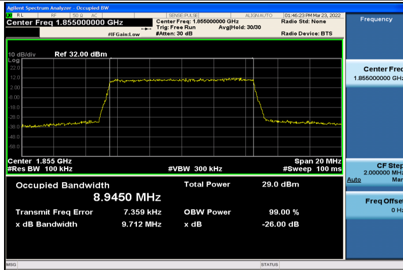
Band2-10MHz-QPSK-18650-50RB#0-8.9450
