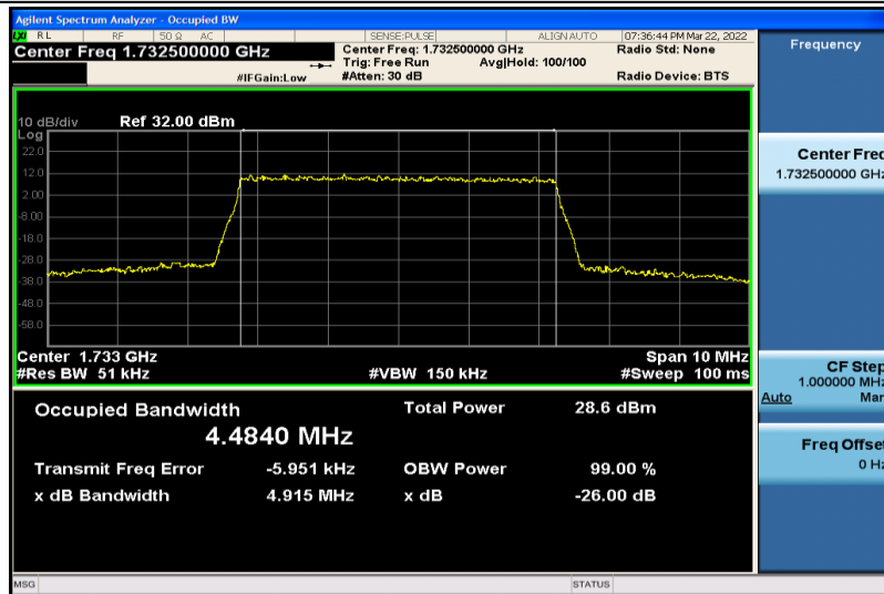
Band4-5MHz-QPSK-17325-25RB#0-4.4840
