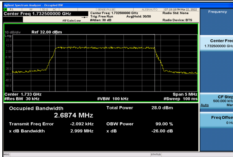
Band4-3MHz-QPSK-20175-15RB#0-2.6874
