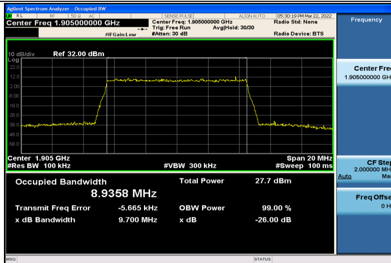
Band2-10MHz-16QAM-19150-50RB#0-8.9358
