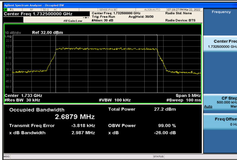
Band4-3MHz-16QAM-20175-15RB#0-2.6879
