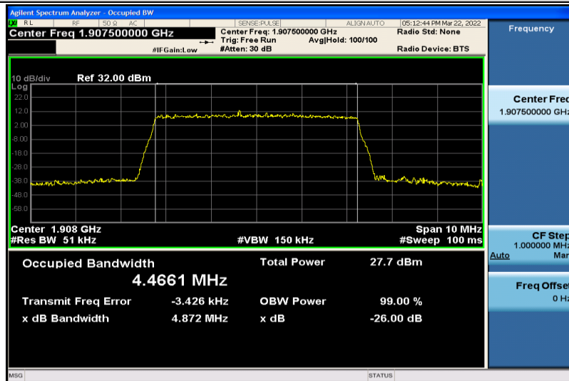
Band2-5MHz-16QAM-19175-25RB#0-4.4661
