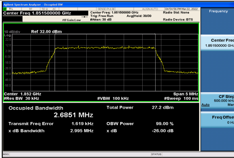
Band2-3MHz-16QAM-18615-15RB#0-2.6851
