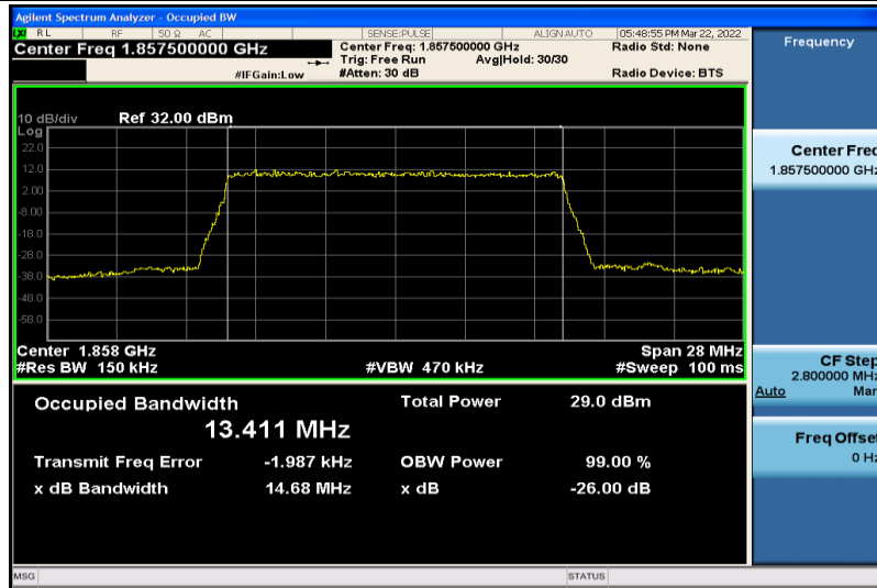
Band2-15MHz-QPSK-18675-75RB#0-13.411
