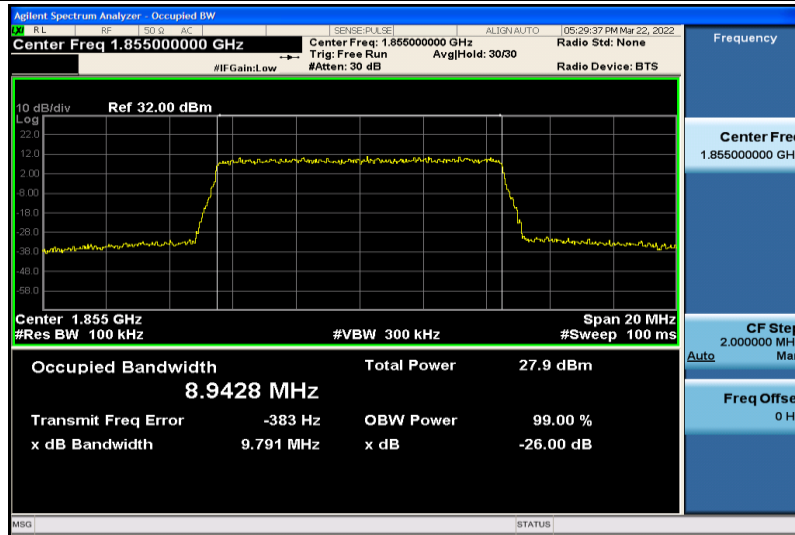
Band2-10MHz-16QAM-18650-50RB#0-8.9428
