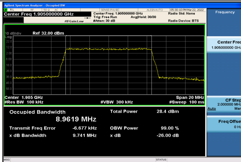
Band2-10MHz-QPSK-19150-50RB#0-8.9619
