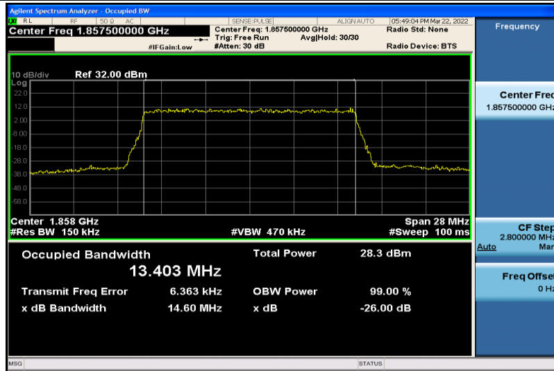
Band2-15MHz-16QAM-18675-75RB#0-13.403
