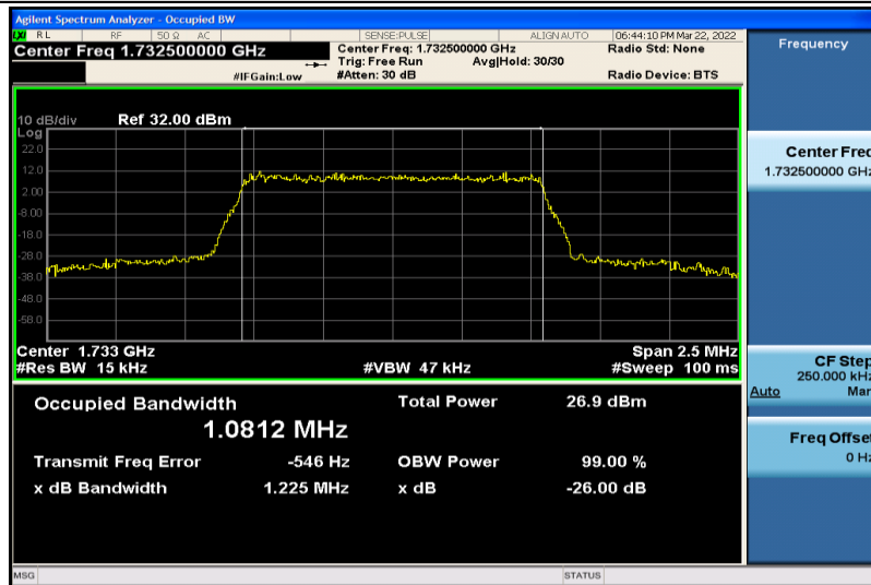
Band4-1.4MHz-16QAM-20175-6RB#0-1.0812
