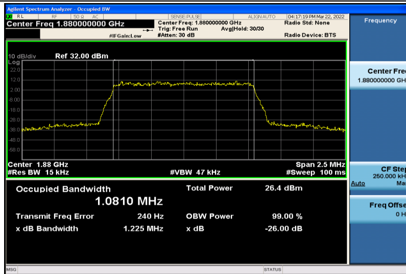
Band2-1.4MHz-16QAM-18900-6RB#0-1.0810
