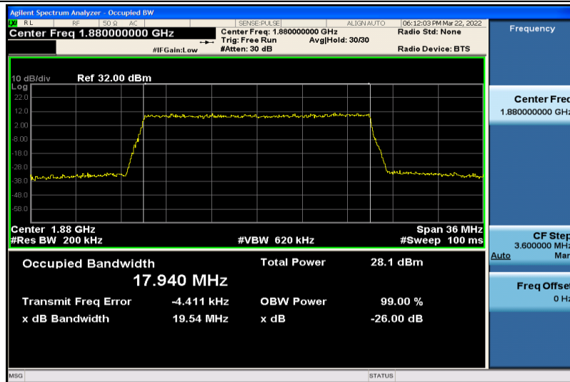
Band2-20MHz-16QAM-18900-100RB#0-17.940
