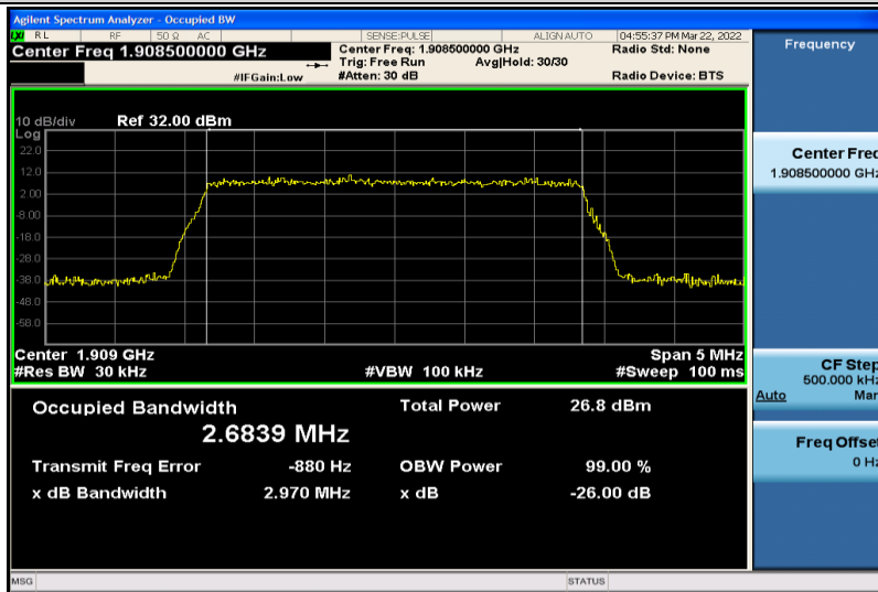
Band2-3MHz-16QAM-19185-15RB#0-2.6839
