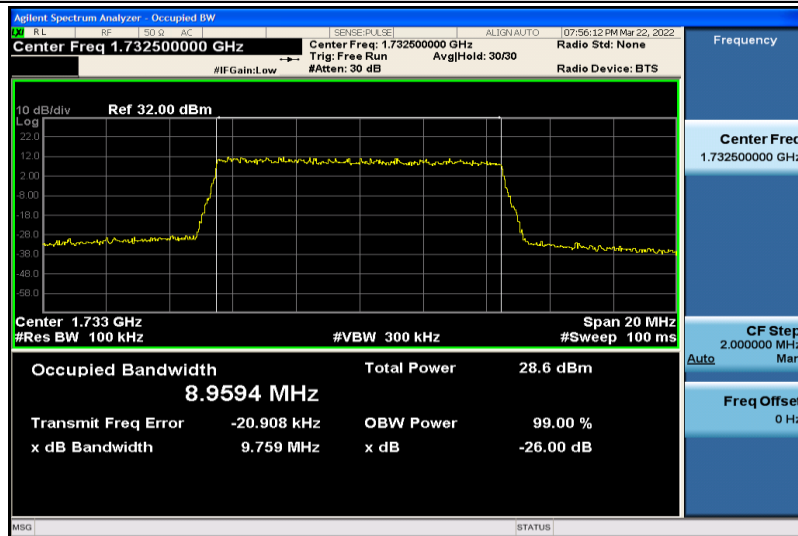
Band4-10MHz-QPSK-20175-50RB#0-8.9594
