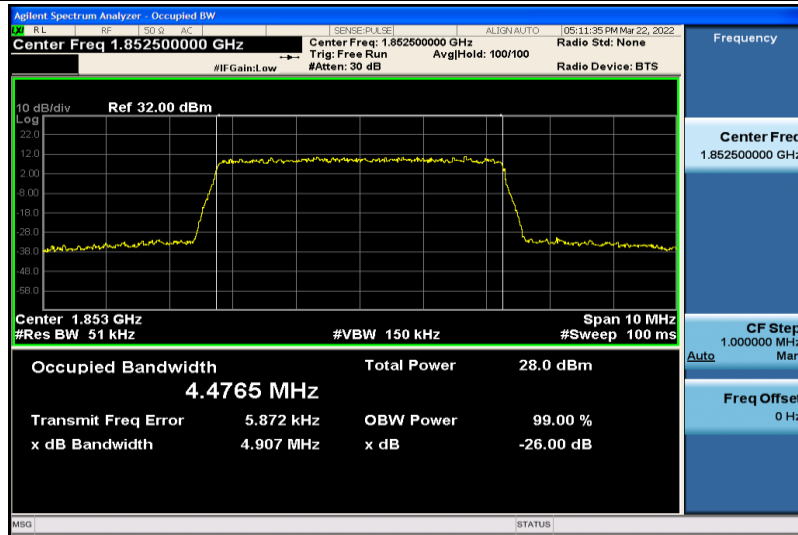
Band2-5MHz-16QAM-18625-25RB#0-4.4765
