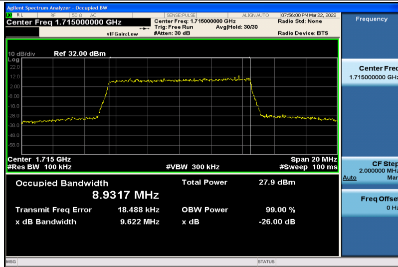
Band4-10MHz-16QAM-20000-50RB#0-8.9317
