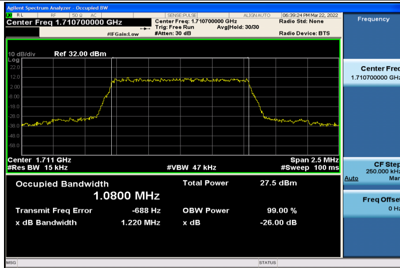
Band4-1.4MHz-QPSK-19957-6RB#0-1.0800
