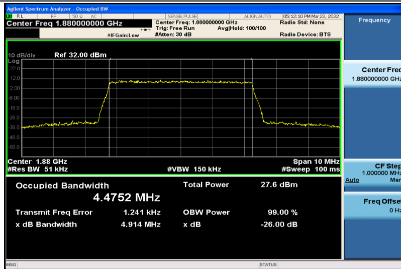
Band2-5MHz-16QAM-18900-25RB#0-4.4752
