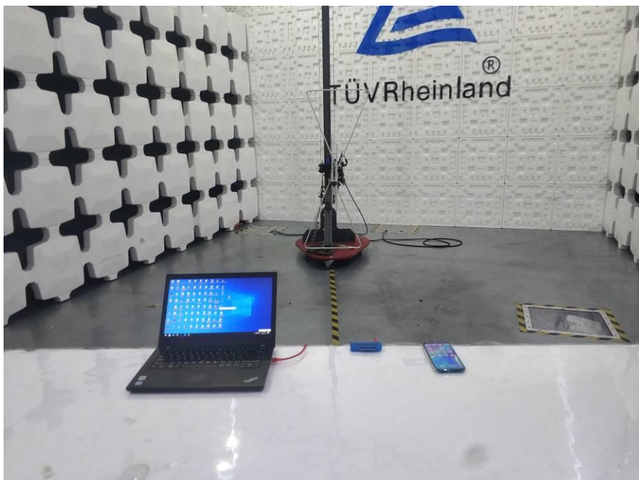
Photograph 4: Set-up photo for Radiated Emission, Below 1GHz
