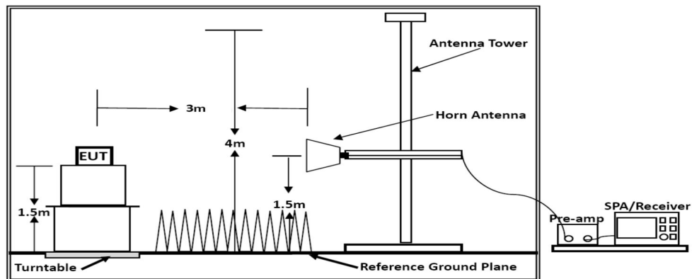
Above 1GHz
