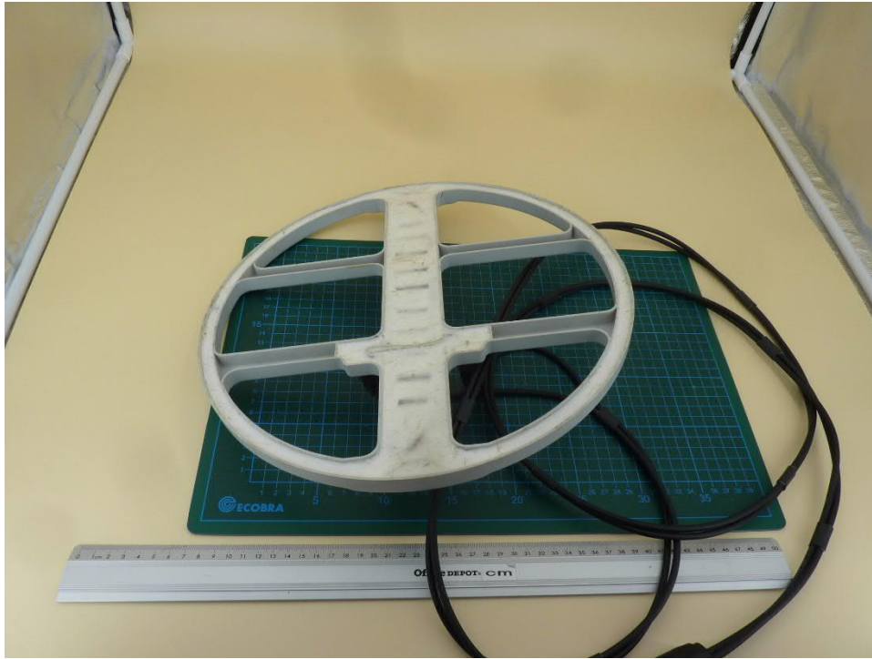
201626_eut13: 35 cm DD-coil bottom view
