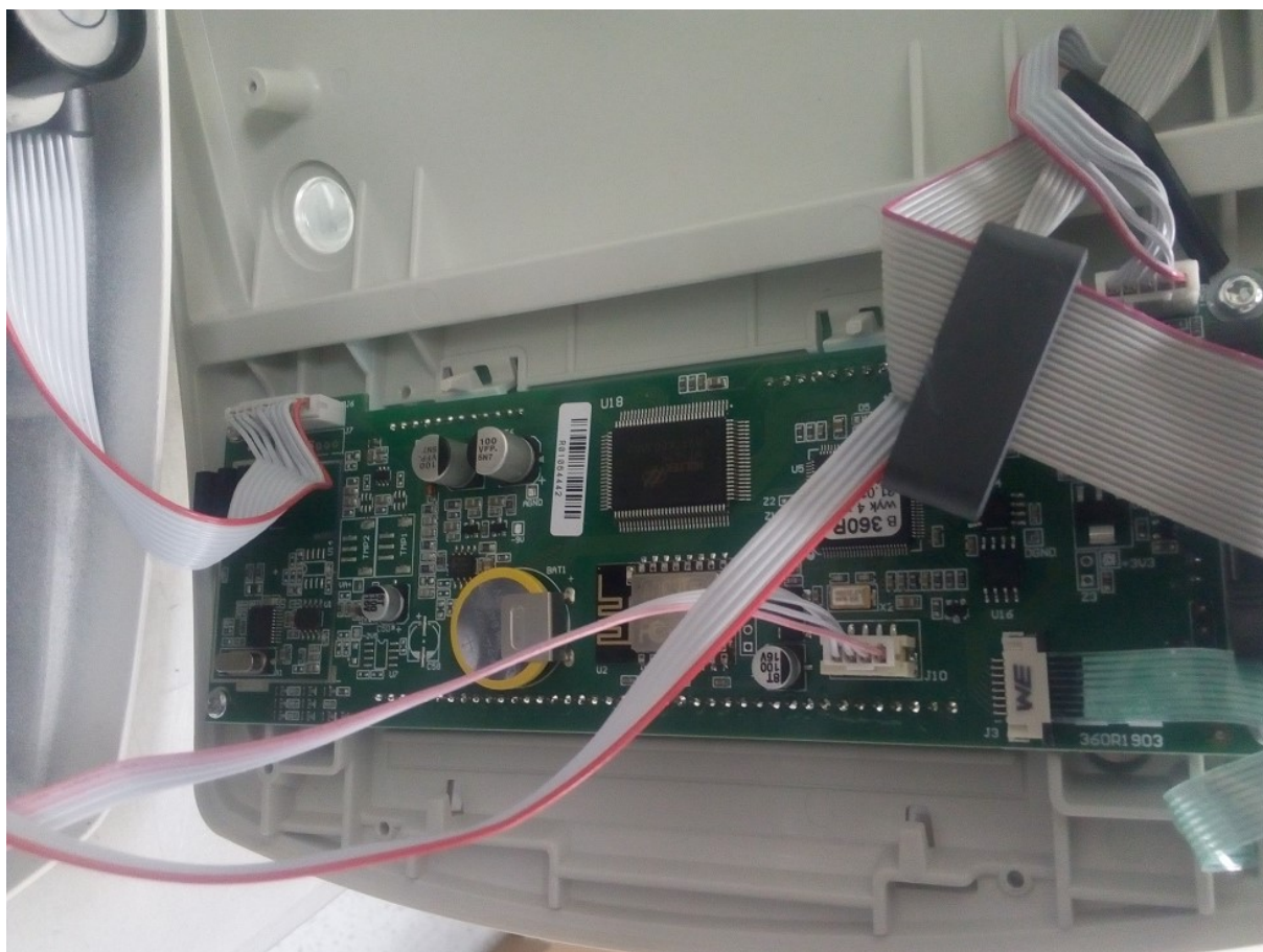
Top housing – PCB under display
