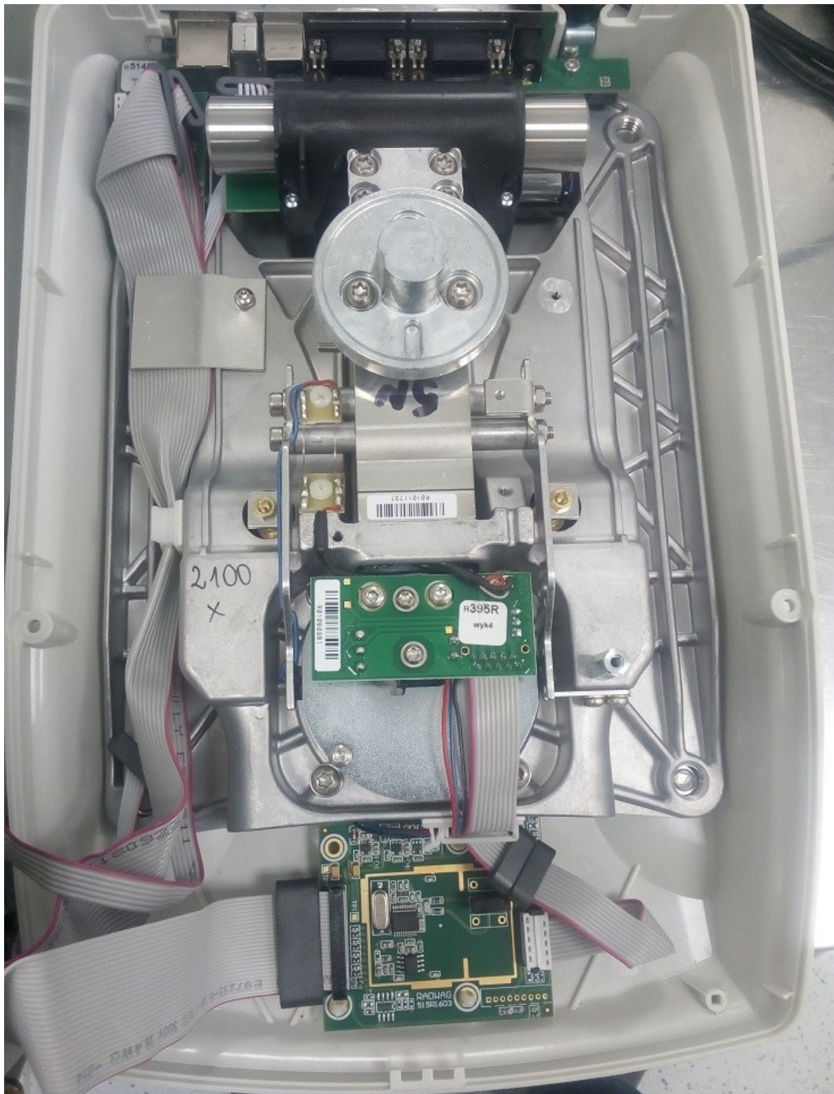
Bottom housing
