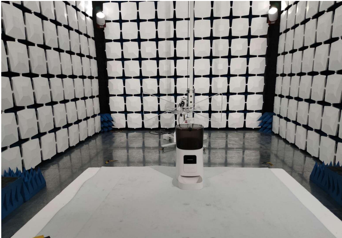
Radiated emission test setup (&lt;1000MHZ)
