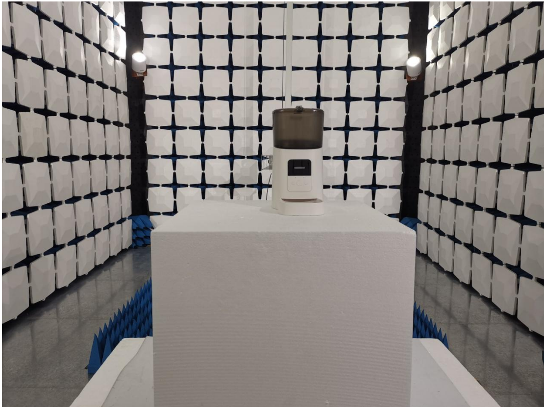
Radiated emission test setup (&gt;1000MHZ)
