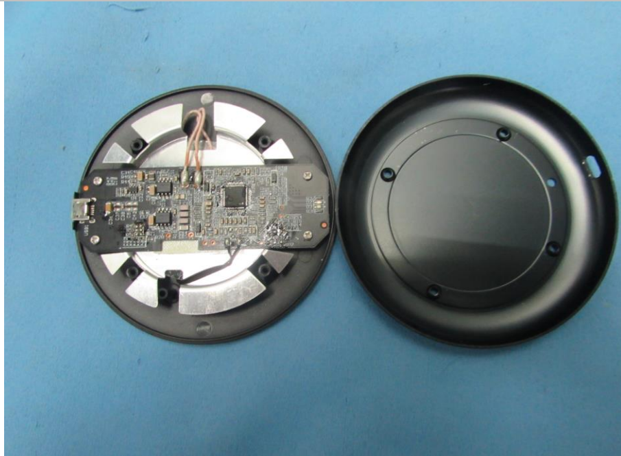
Internal view
