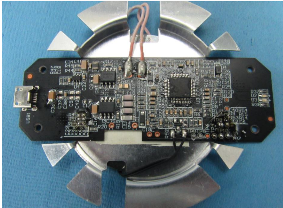
PCB view
