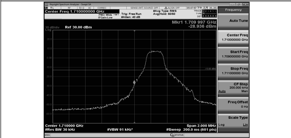
Band4-1.4MHz-QPSK-19957-6RB#0
