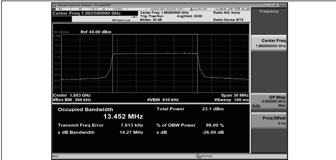
Band25-15MHz-QPSK-26615-75RB#0-13.438
