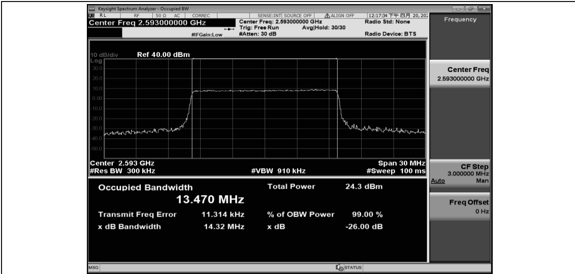
Band41-15MHz-16QAM-41515-75RB#0-13.470
