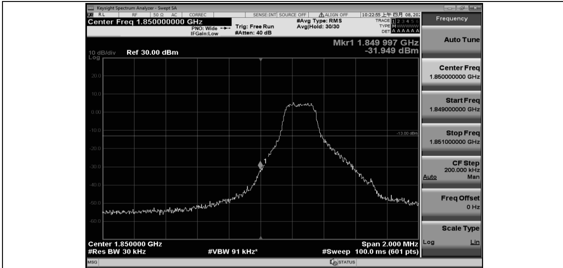
Band2-1.4MHz-16QAM-18607-1RB#5
