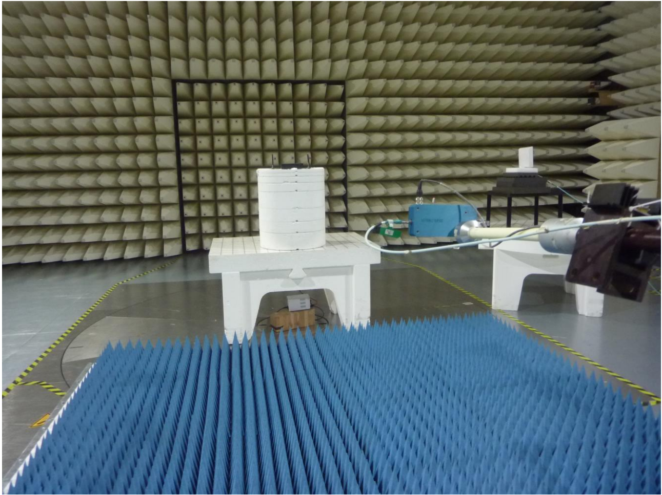
Figure 19: Test Setup for Radiated Emissions 18GHz to 26 GHz (BT LE and Licensed Modes)
