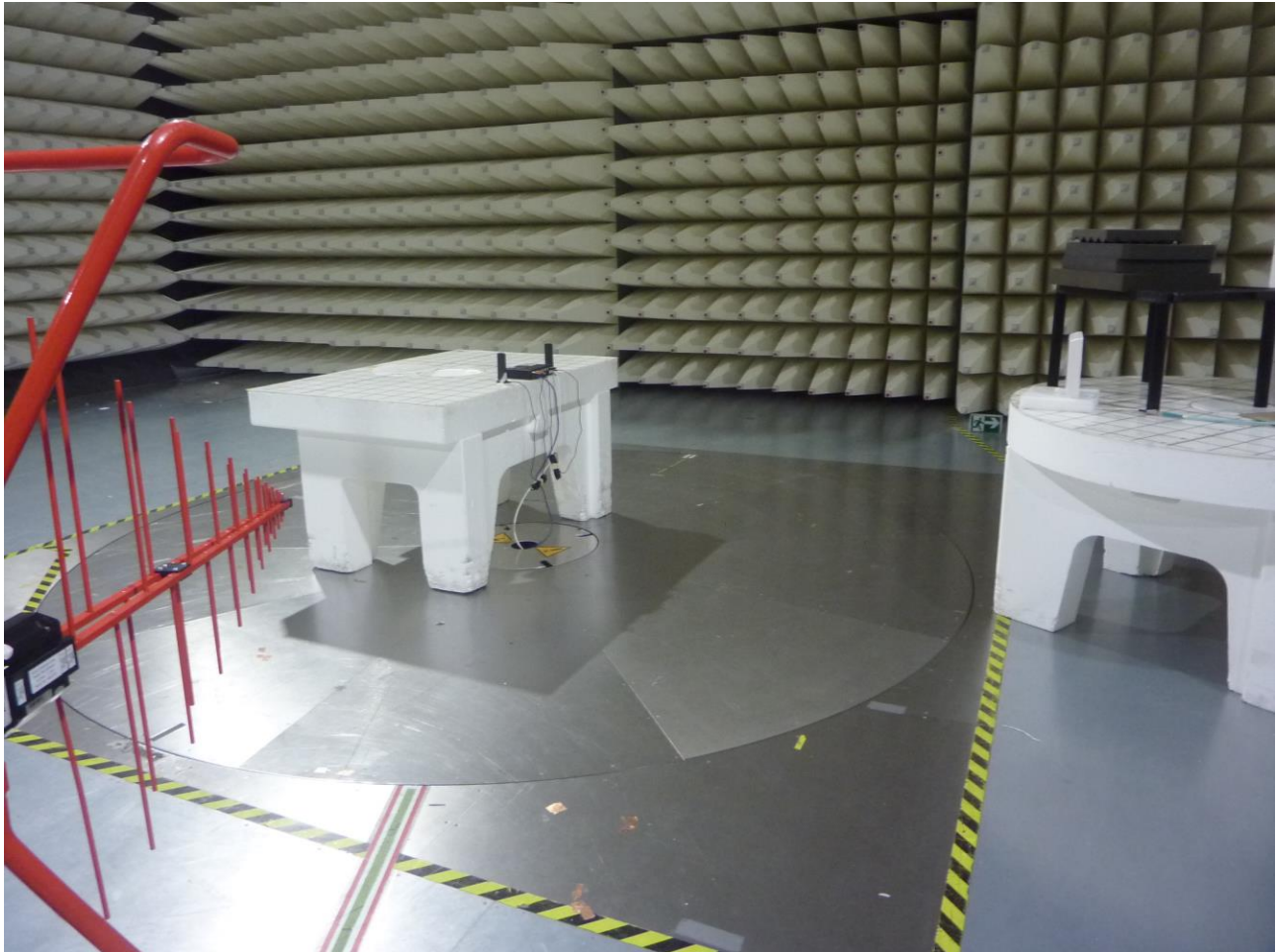
Figure 17: Test Setup for Radiated Emissions 30MHz to 1000MHz (BT LE and Licensed Modes)
