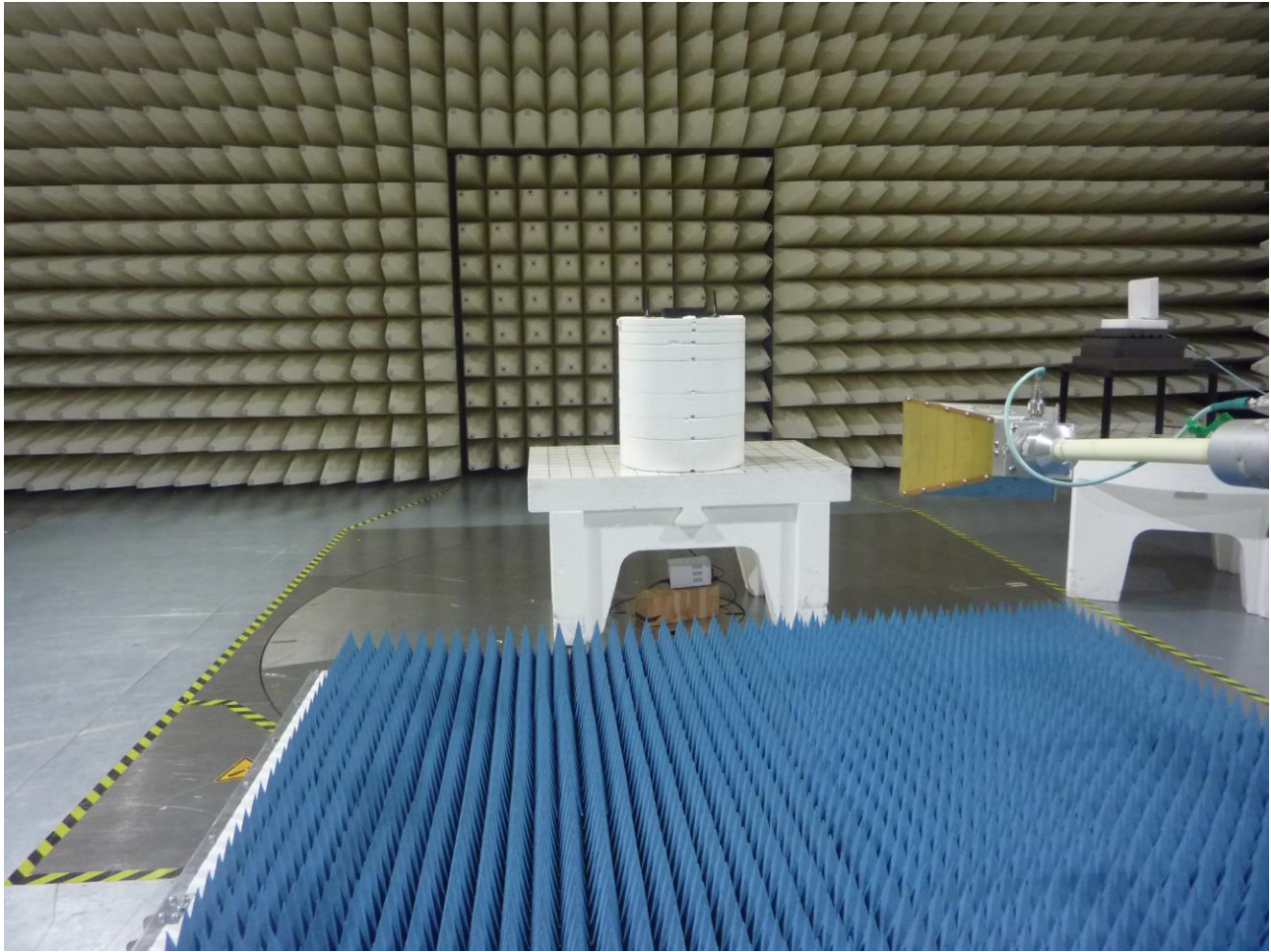
Figure 18: Test Setup for Radiated Emissions 1GHz to 18GHz (BT LE and Licensed Modes)
