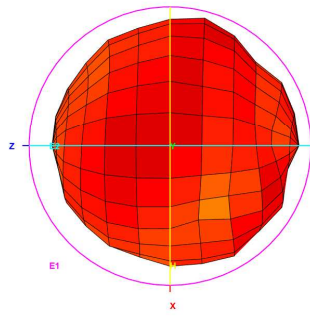
Total_3D_Left View_1.8GHz
