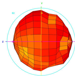
Total_3D_Left View_1.9GHz
