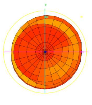
Total_3D_Side View 1_900MHz
