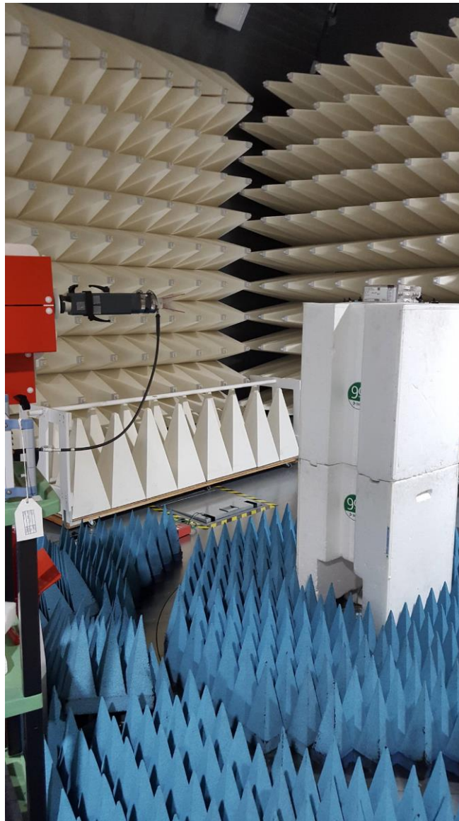
Figure B3. High Range Radiated Emission test setup 18-40GHz
