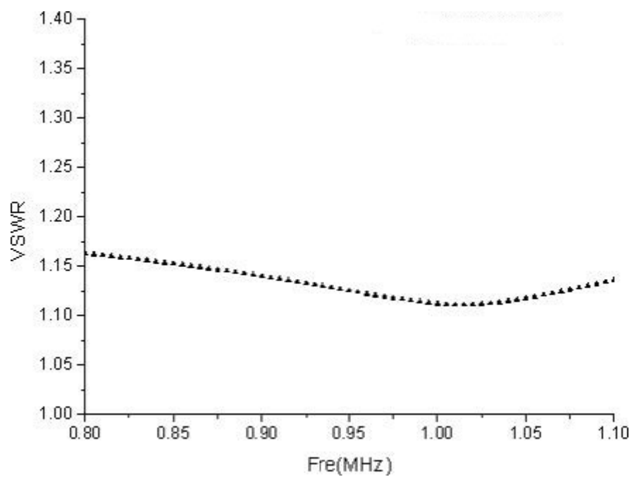
③ Antenna standing wave VSWR test diagram
