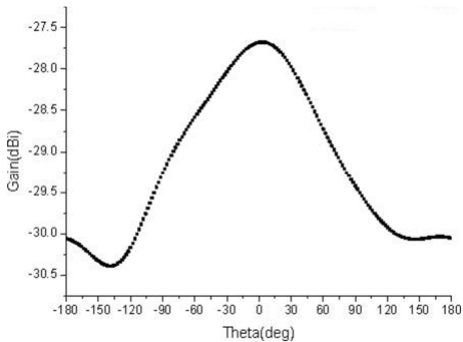
② Antenna gain test diagram (Fre=920MHz)
