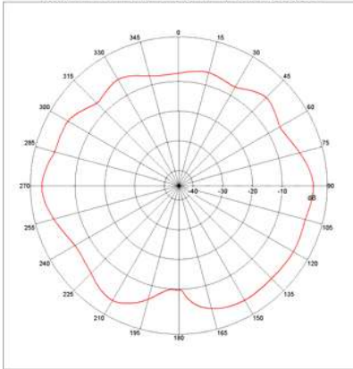
Far-field Power Distribution(H+V) on Y-Z Plane Plot Peak Gain(H+V)= 1.11 dBi; Plot AvgGain(H+V)= -2.96dBi @2.44000 GHz
