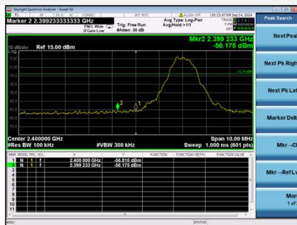
GFSK (BLE 1Mbps) LOW CHANNEL, BAND EDGE
