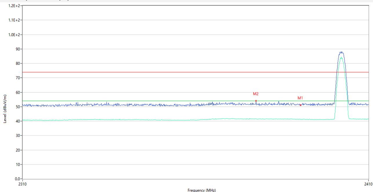
GFSK (BLE 1Mbps) CH0 ANT V
