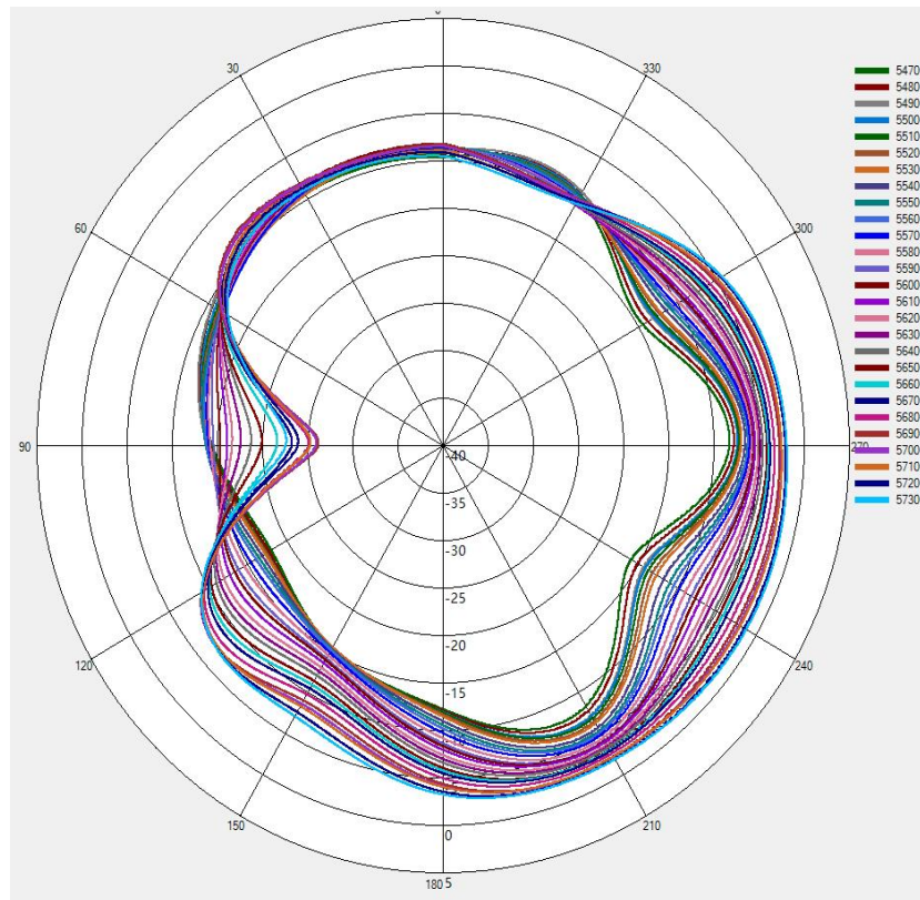
(13) X-Y Plane(unit:dBi)
