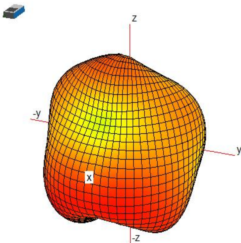
(4) Typical Free Space 3D Radiation Pattern at 2.5GHz(unit:dBi):
