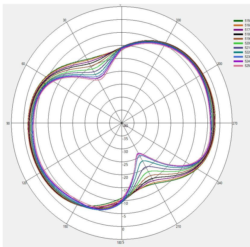
(6) X-Z Plane(unit:dBi):
