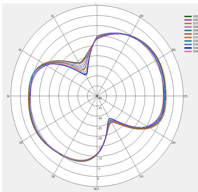
(10) X-Z Plane(unit:dBi):
