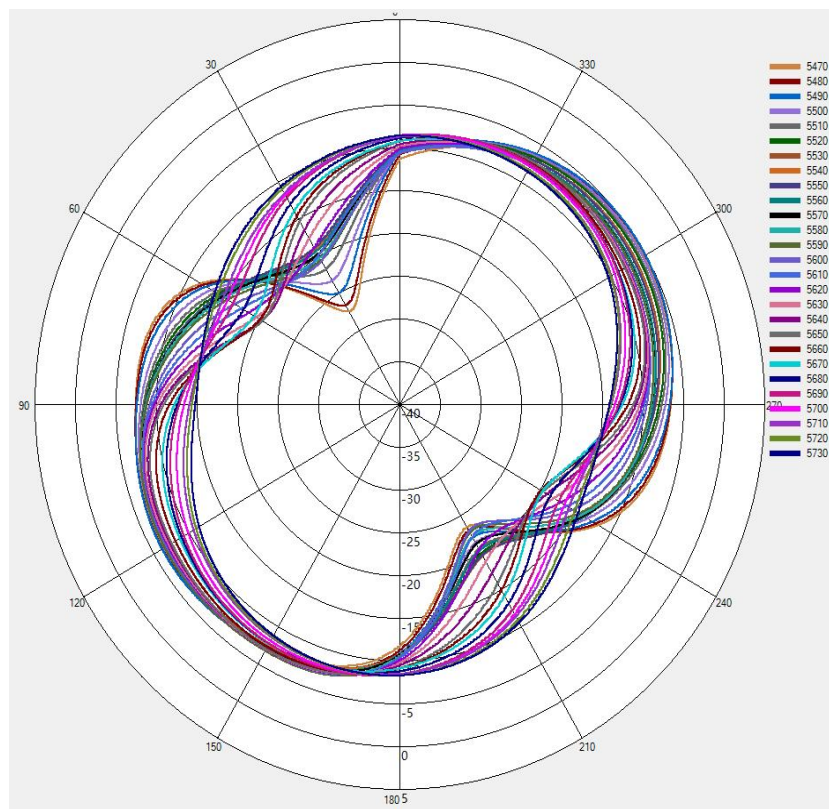
(14) X-Z Plane(unit:dBi):
