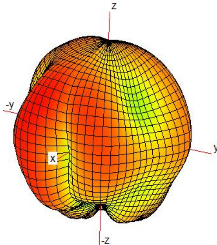
Typical Free Space 3D Radiation Pattern at 5.25GHz(unit:dBi): (12)
