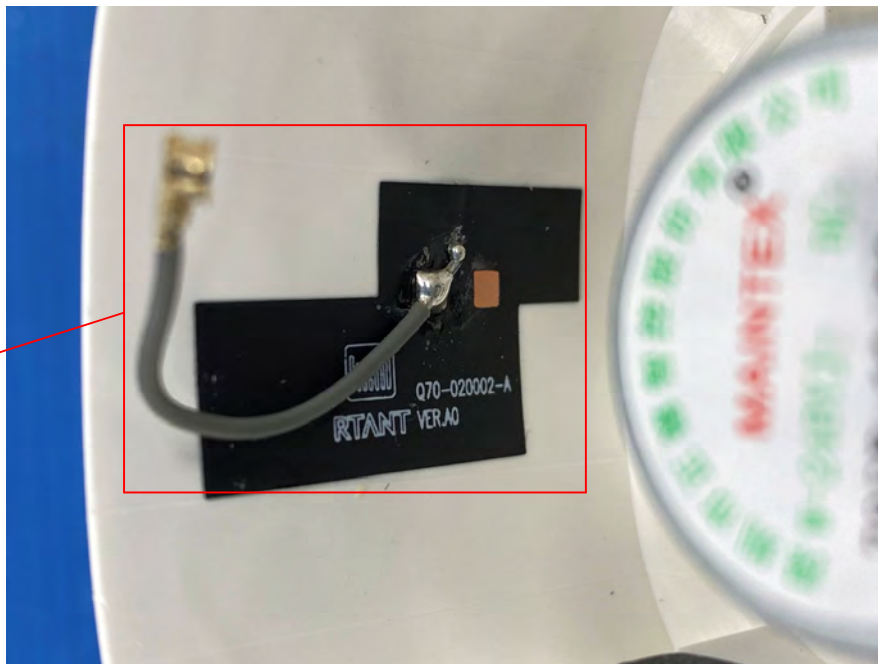
FPC antenna
