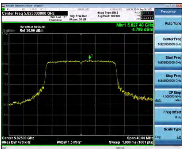
U-NII-3, 802.11ax HE20, Channel No.: 165
