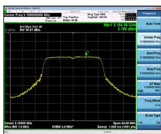
U-NII-1, 802.11n HT20, Channel No.: 36
