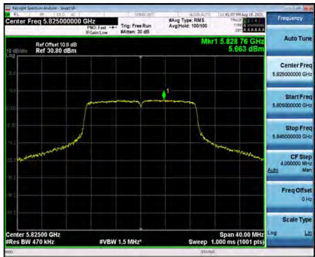
U-NII-3, 802.11ac VHT20, Channel No.: 165
