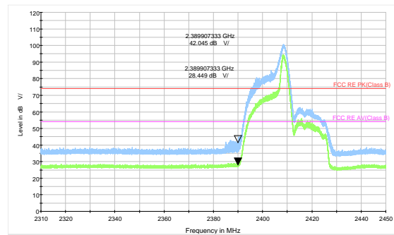
802.11n HT40 -Channel 2 Peak + Average
