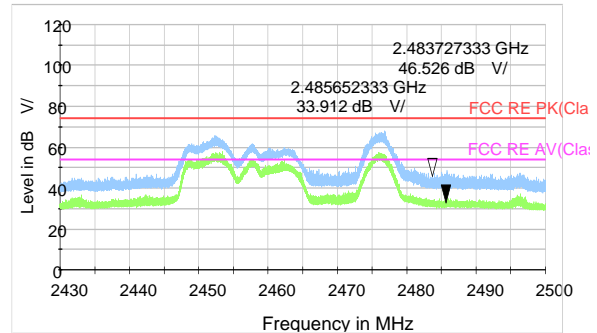
802.11n HT40 -Channel 10 Peak + Average
