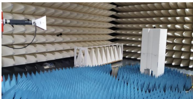
Figure B7. Radiated emission Test Setup 2
