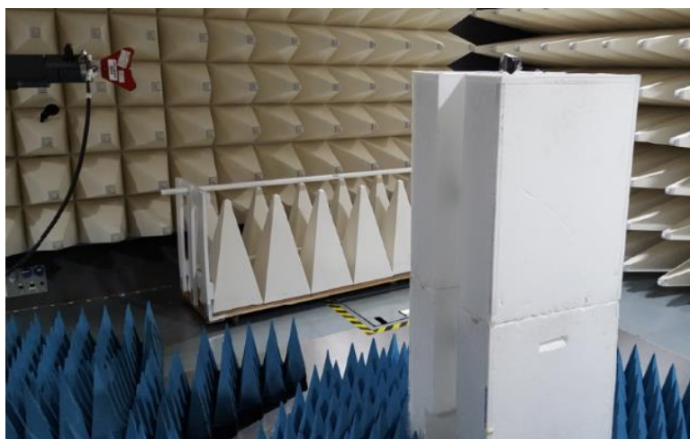
Figure B8. Radiated emission Test Setup 3
