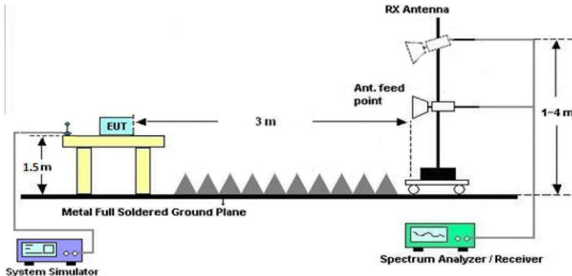
Figure 3. Above 1 GHz
