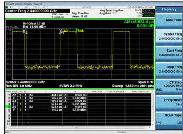
GFSK(BLE 2Mbps)
