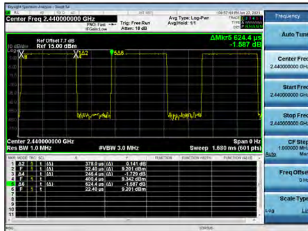
GFSK(BLE 1Mbps)
