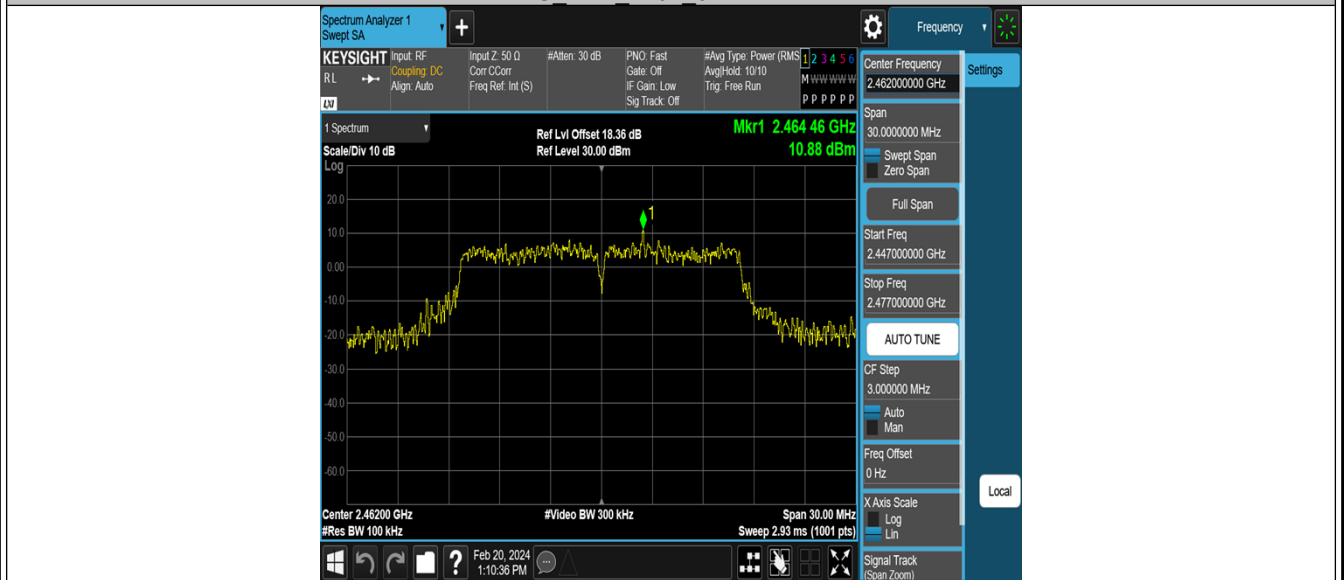
11G Ant1_2462_30~1000
