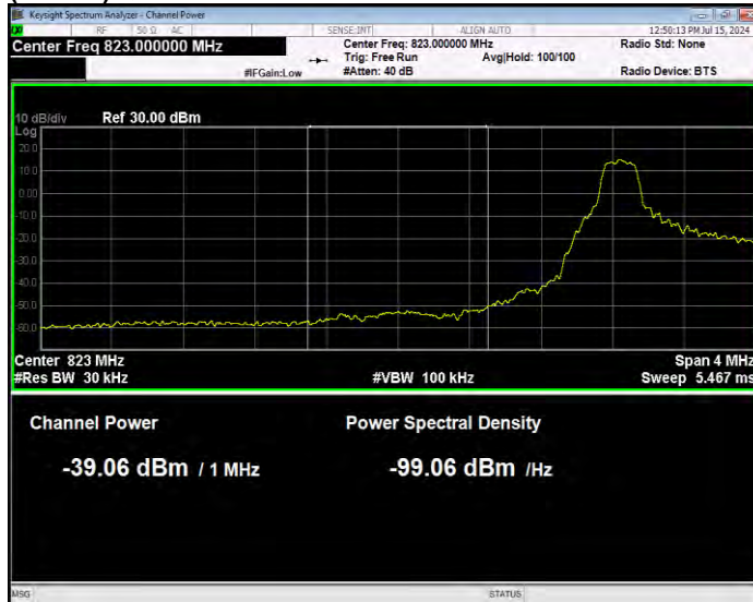
Band26(824-849) QPSK BW=3MHz Channel=26805 RB Size=1 Position=#0 Extended
