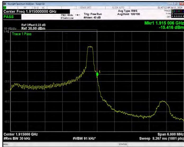
Band25 QPSK BW=3MHz Channel=26675 RB Size=15 Position=#0 Extended
