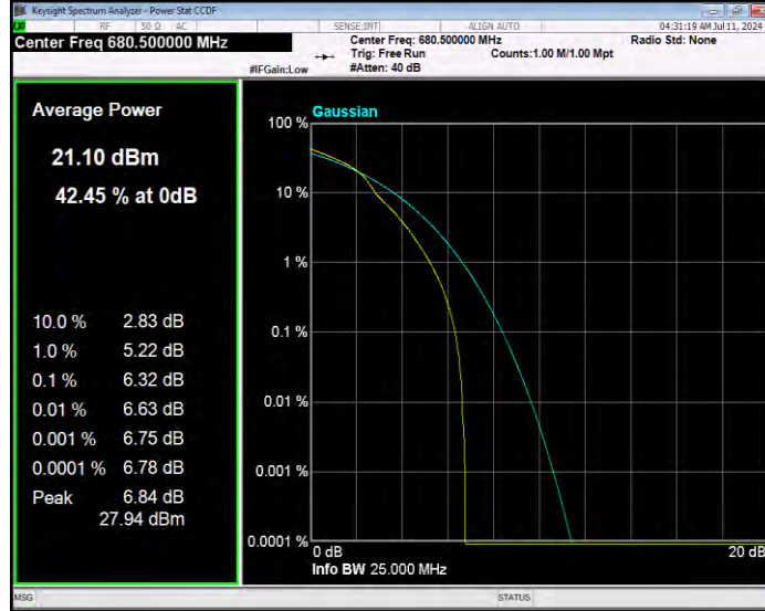
Band71 16QAM BW=5MHz Channel=13347 RB Size=1 Position=#0
