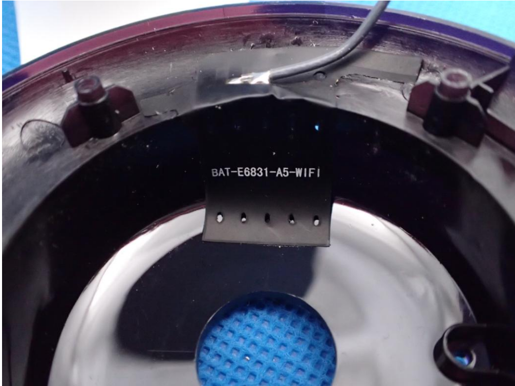
WIFI ANTENNA
