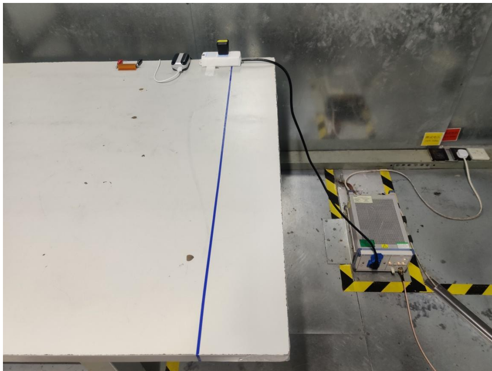
Conducted Measurement Photos(I09)
