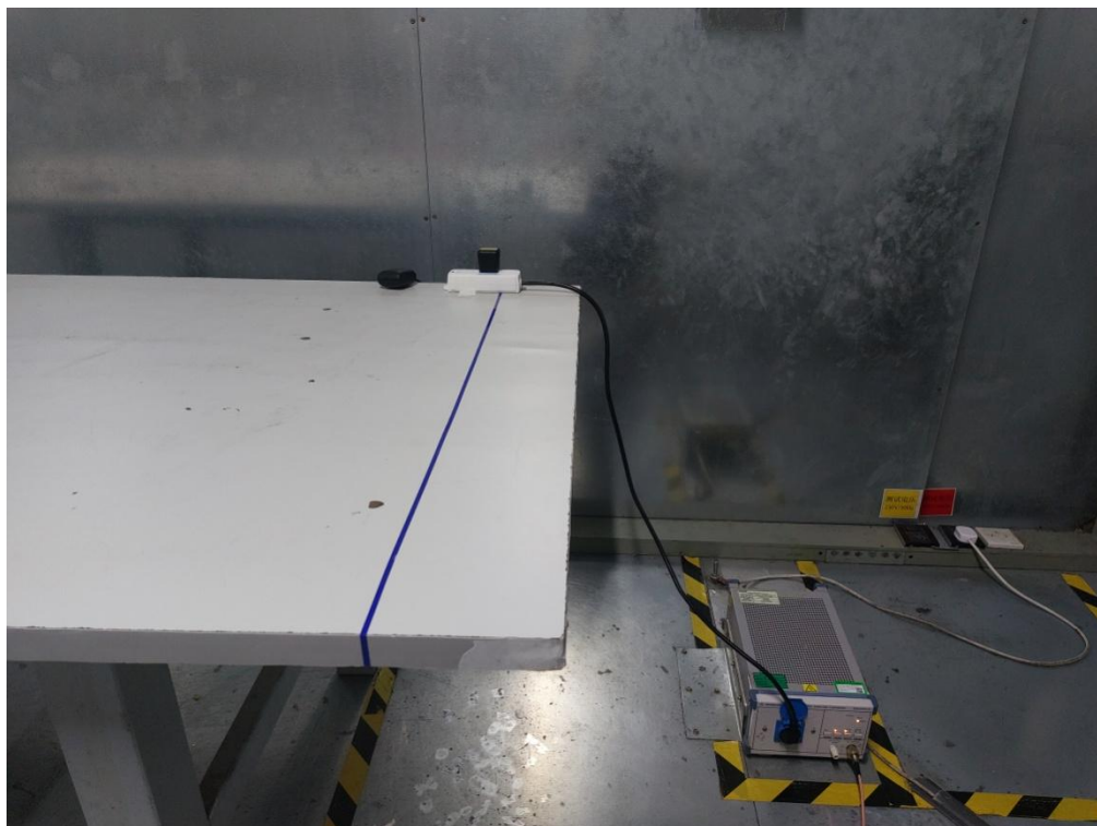
Conducted Measurement Photos(I11)
