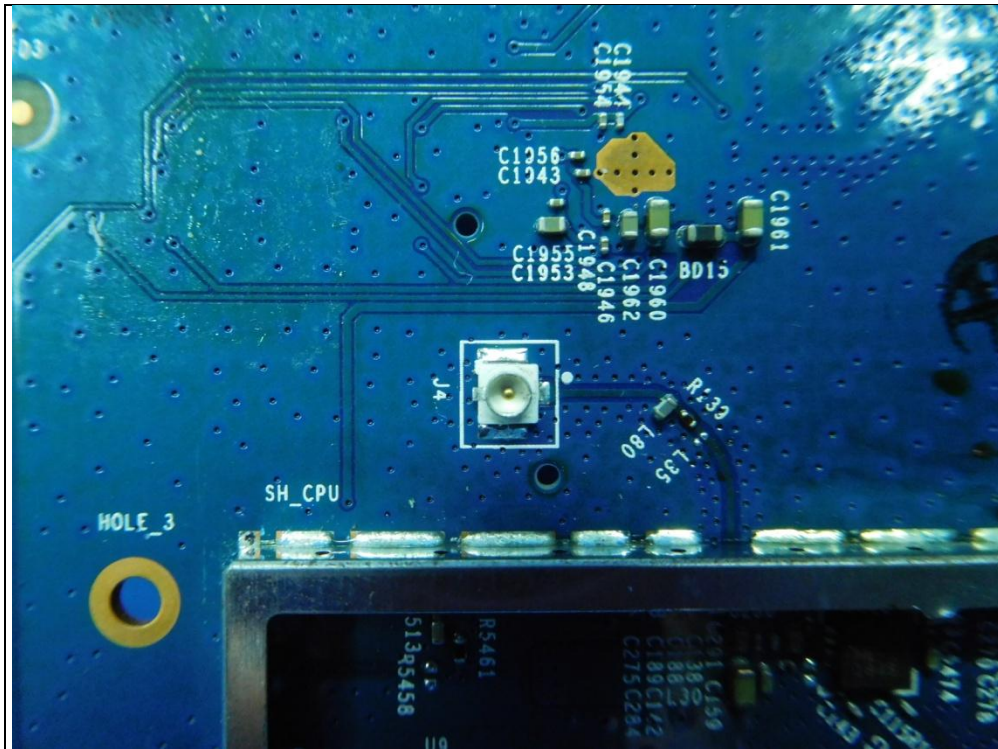
WLAN Antenna 1
